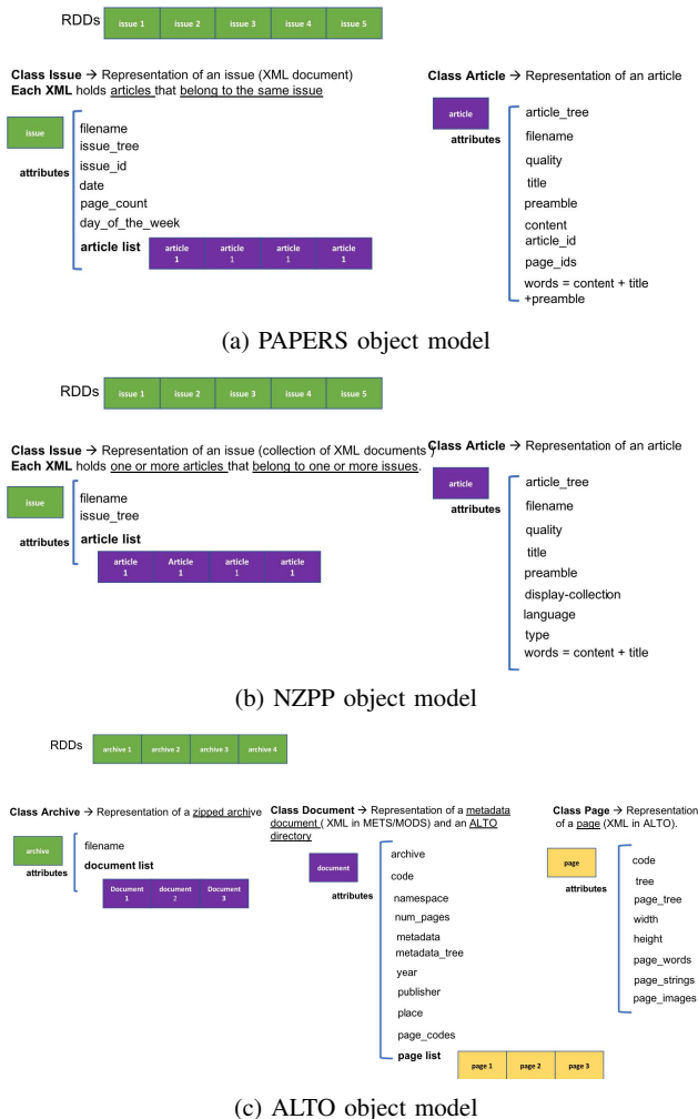
Fig. 3: Object models available in defoe
