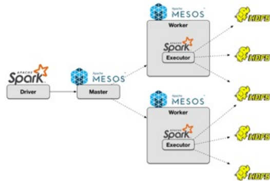
Fig. 13: Apache Spark Architecture in Urika-GX .
