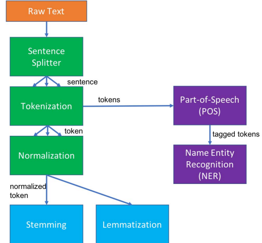
Fig. 4: defoe NLP preprocessing pipeline implemented.
