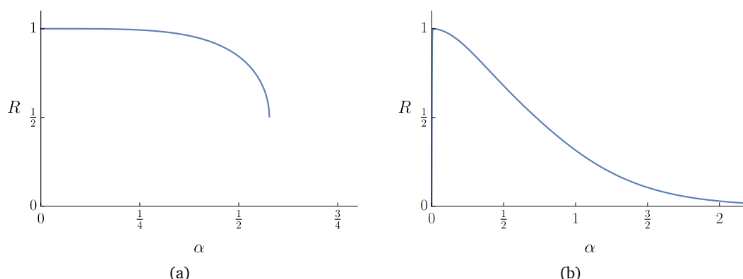
Fig. 4: Ratios R plotted as a function of the ratio of the two circle lengths \alpha = L_1/L_2 for (a) a Holographic CFT, (3.20), and (b) for a free boson where we summed (3.22) up to l = 200 . The fact that R shoots up near \alpha = 0 in (b) is a consequence of this finite sum.
