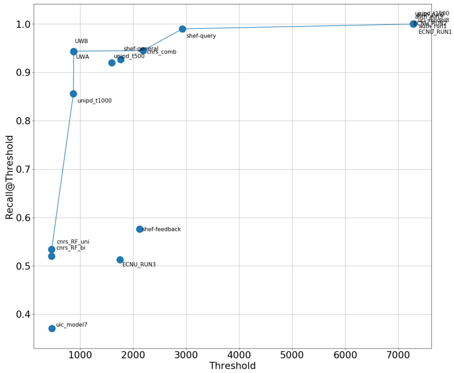
Fig. 7. Recall at the threshold rank as a function of the number of abstracts shown to the user.
