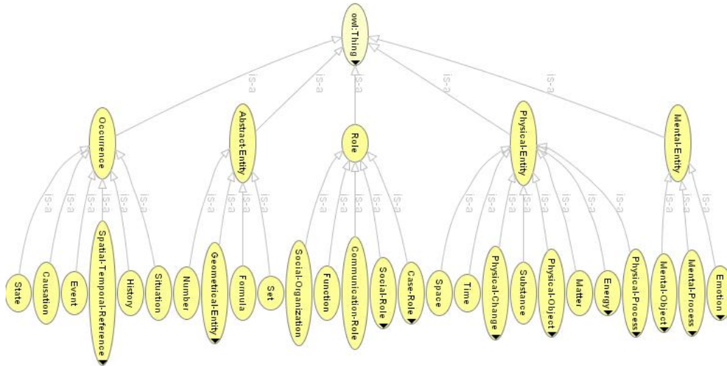
Figure 4: LRI-Core, first two layers
