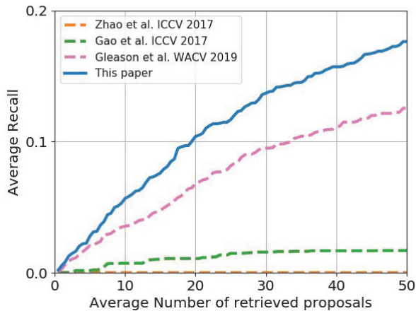
Figure 7: Temporal comparison of interactivity proposals versus regular action proposals under varying number of retrieved proposals. Modeling interactivity rather than activity is beneficial.
