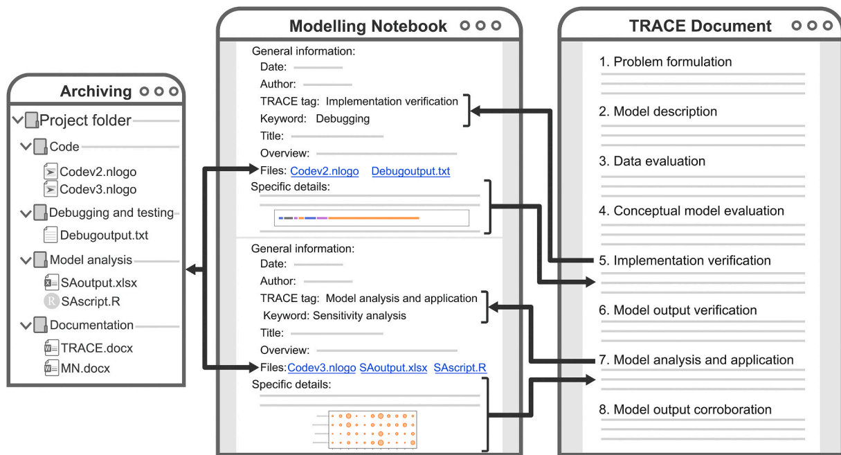
Fig. 2. Schematic figure explaining the relation between files in a modelling project, a modelling notebook, and TRACE. Notebook entries are added chronologically with tags provided by the terminology from the TRACE framework. Standardized tags and keywords, in turn, facilitate the compilation of a TRACE document from the specific details included in the notebook entries. Entries provide hyperlinks to all files related to a modelling task, indicating their location in the archiving system; TRACE terminology should also be used to organize and name files and folders.
