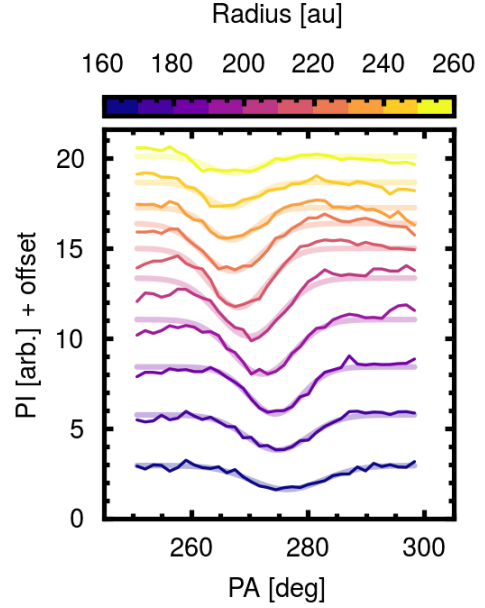
Fig. 6. Azimuthal profiles of the western shadow at different (deprojected) radial bins between 160 and 260 au. The smooth, shadowed lines correspond to the best-fit Gaussian profiles, respectively.
