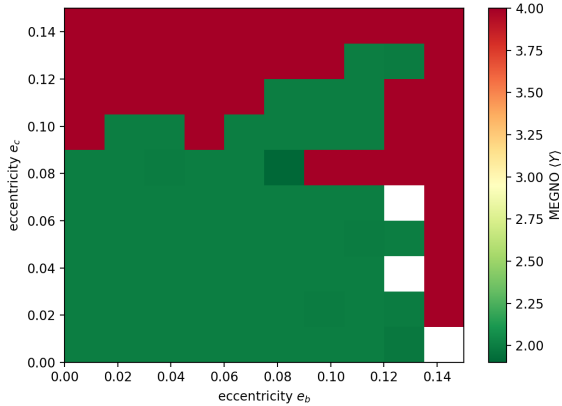
Figure 8. As Fig. 7, but on a 1 Gyr timescale. We have not plotted orbits with e > 0.15 , as they are all chaotic on this timescale.
