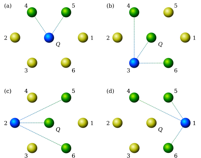
FIG. 8. The four steps realizing the Steane code using \text{CNOT}^n gates. Green spheres (spheres with one connection) represent target qubits, i.e., qubits on which the NOT operation is performed, blue spheres (spheres with multiple connections) are control qubits, and the yellow spheres (unconnected spheres) represents idle qubits. The four steps (a)–(d) corresponds to the four gates in Fig. 7.
