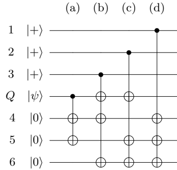
FIG. 7. Encoding scheme for the Steane code. Qubit Q is initially in state |\psi\rangle and the circuit encodes it into a seven-qubit state using one \text{CNOT}^2 gate and three \text{CNOT}^3 gates. The first three qubits are prepared in the state |+\rangle = (|0\rangle + |1\rangle)/\sqrt{2} , while the last three qubits are prepared in the state |0\rangle .
