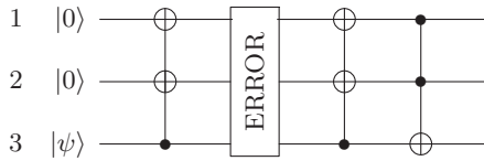
FIG. 5. Effective three-qubit error correction code using two \text{CNOT}^2 gates and a Toffoli gate. We label the top qubit 1, the middle qubit 2, and the lowest qubit 3. Note that the figure is shown with regular Toffoli gates, while our simulation is done with the i -Toffoli gates; however, it does not change the result.
