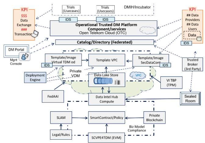
Figure 2. Trusted Data Market functional components
