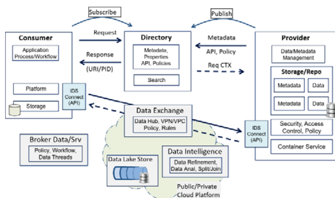
Figure 1. Data Market infrastructure components leveraging IDS Architecture 2.0.
