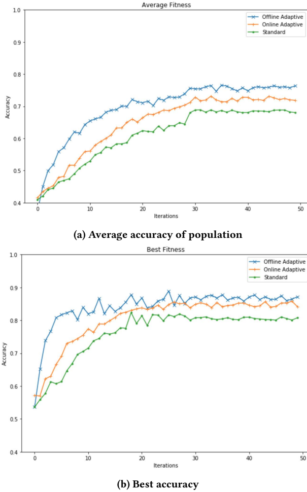
Figure 6: Training curves. Average accuracy refers to the average performance of whole population at the given optimization iteration. Best accuracy refers to best found performance of an individual model from the population.
