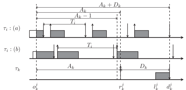
Fig. 7. The densest possible packing of jobs of \tau_i with carry-in job. Case (a): D_i \leq D_k \wedge S_i > C_k^* , Case (b): D_i > D_k \wedge S_i \leq C_k^* .
