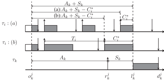
Fig. 8. The densest possible packing of jobs of \tau_i with carry-in job. Case (a): D_i \leq D_k \wedge S_i \leq C_i^* , case (b): D_i > D_k \wedge S_i < C_i^* .
