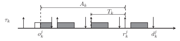
Fig. 3. The densest possible packing of jobs of \tau_i without carry-in job, if i = k .
