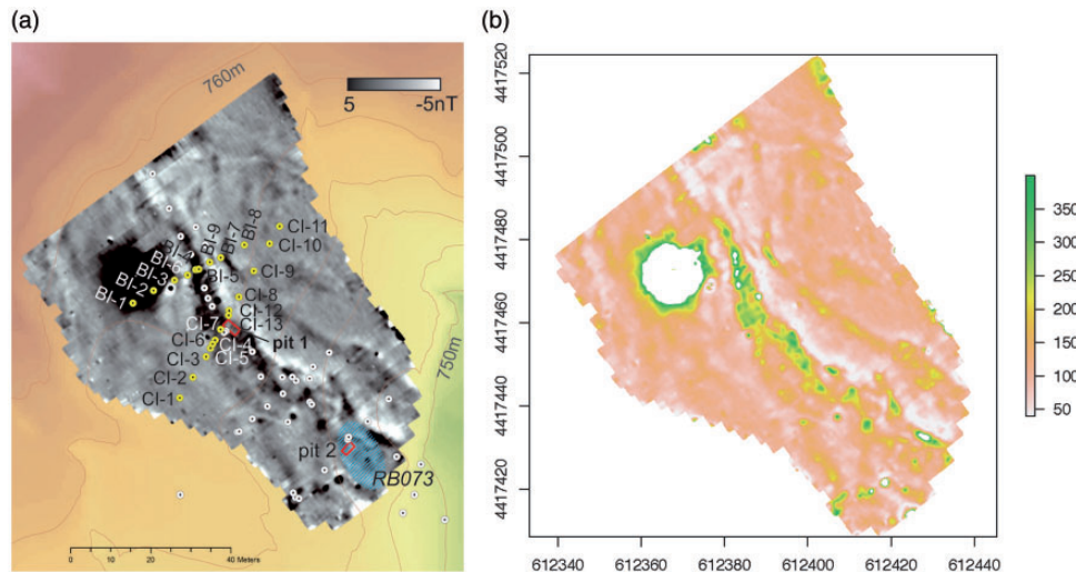
Figure 4. (a) Magnetic gradiometry map of the area of study. Black dot at BI-1/2 is because of the presence of a small electric power station interfering in the signal. Small dots indicate location of corings. (b) Derived map showing depth to regolith in centimetres, based on observed optimal statistical relation between signal strength and 'true depth to regolith'.
