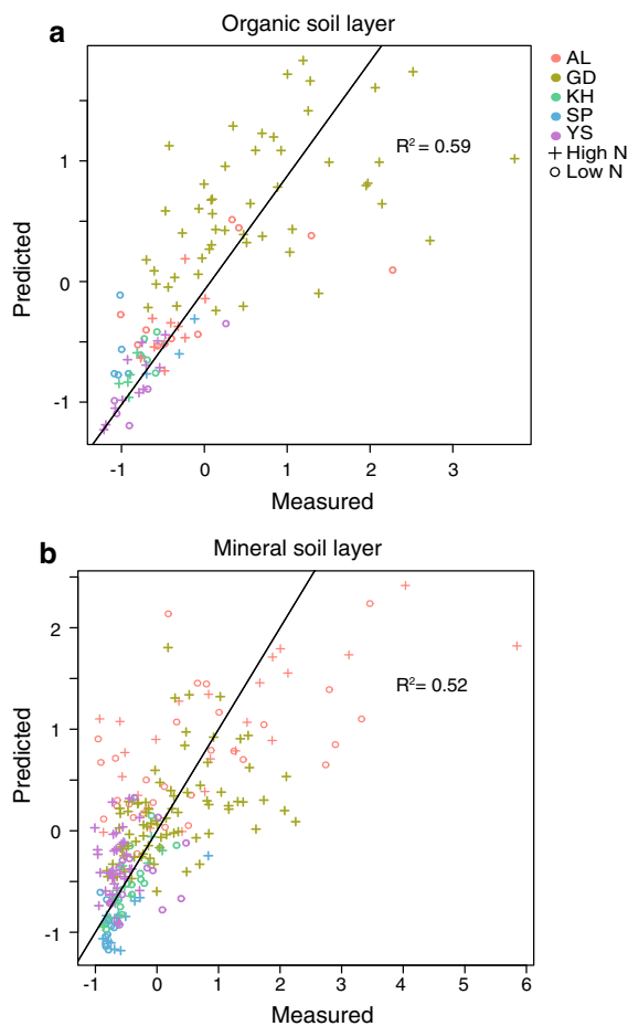
Fig. 4 Partial least squared regression (PLS-R) model output and 1:1 line. The predicted values of ^{15}\text{N} recovery are given on the y-axis and the measured ^{15}\text{N} recovery values on the x-axis for the organic (a) and mineral (b) soil. The ^{15}\text{N} recovery (%) data is z transformed prior to the analysis
