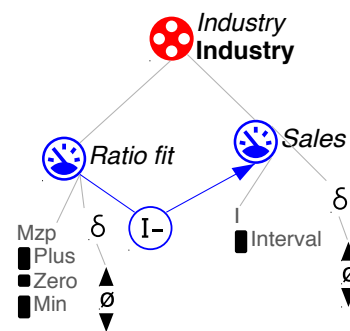
Figure 4. Ratio fit on Sale.
