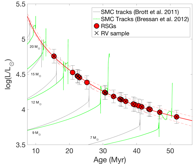
Fig. 7. Luminosity-age diagram for all RSGs in NGC 330, stars that have RV measurements from the present study are marked with a cross. Luminosities are derived the J -band magnitude calibration of Davies et al. (2013). Using the least luminous RSGs, we estimate the age of the NGC 330 to be 45 \pm 5 Myr. SMC-like evolutionary tracks from Brott et al. (2011) are used to estimate ages, and Bressan et al. (2012) tracks are shown to highlight differences between models.
