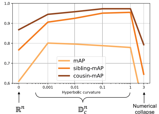
Figure 4: Effect of hyperbolic curvature on the hierarchical action search performance of Hierarchical-ActivityNet. We report sibling- and cousin-mAP, as well as standard mAP. For c = 0 , the space collapses to a Euclidean space, which hurts the scores. For large curvatures, results drop due to numerical instabilities. We recommend a hyperbolic space with 0 < c \leq 1 .
