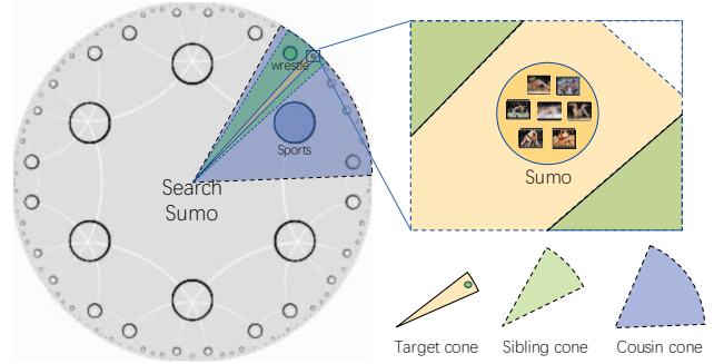
Figure 3: Hierarchical action search. For an action query, we start our search from the projection in the hyperbolic space and expand the entailment cone of the query in all directions. Upon enlarging the entailment cone, we first absorb videos from sibling action cones, then cousin cones. Only afterwards, we retrieve actions from other cones.
