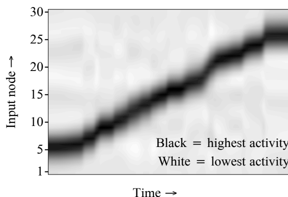
Figure 7: Reflection after 30,000 pieces of data: overtrained behaviour.
