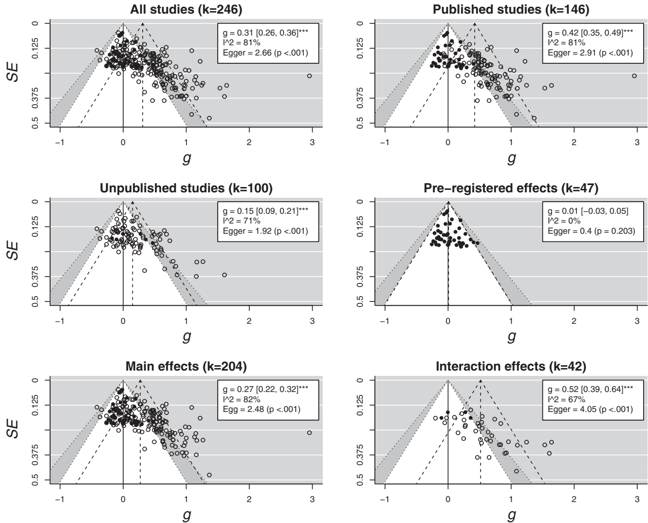
Figure 1. Funnel plots of all studies, published studies, unpublished studies, preregistered studies, main effects, and interaction effects. g = Hedges' g random effects model estimate (center of dotted funnel), including 95% confidence interval. I^2 = heterogeneity measure; Egger = Egger's test regression coefficient and p value; The white- and gray funnel represent a 95% and 99% confidence level, respectively. Black dots represent preregistered studies. *** p < .001 .
