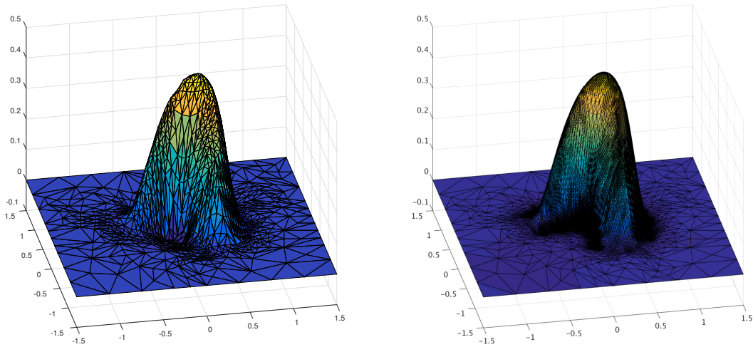
Figure 2: Approximations u_{\tau_i, K}^{\lambda_{\sigma_i}^{(K-1)}} for i = 3 (left) and i = 6 (right) produced with K = 6 , \zeta = \sqrt{2} , \theta = 0.1 .
