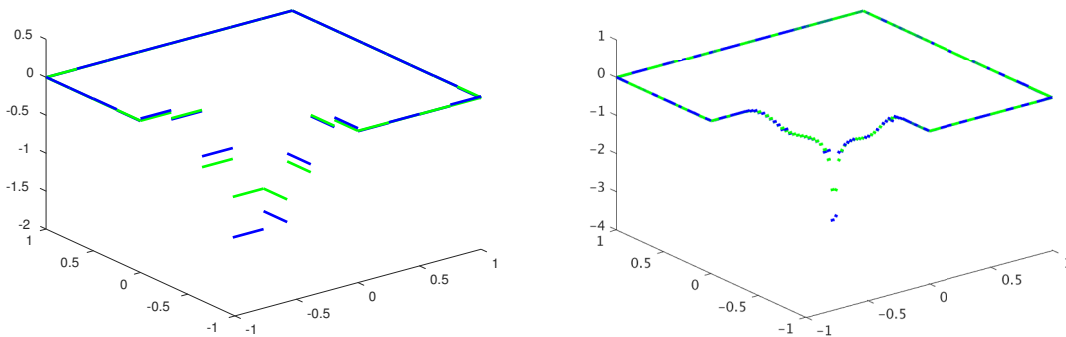
Figure 3: Comparison between \lambda_{\sigma_i}^{(K-1)} (blue) and the L_2(\gamma) -orthogonal projection of \lambda onto \mathcal{A}_{\sigma_i} (green) for i = 3 (left) and i = 6 (right).
