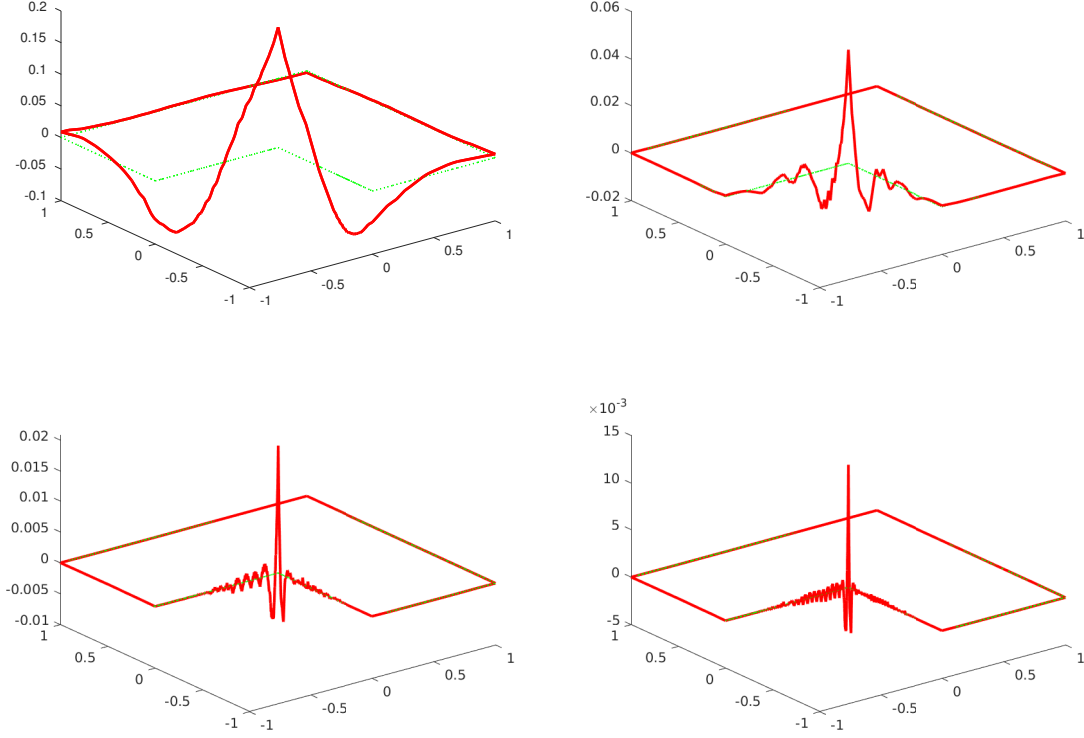
Figure 4: Traces u_{\tau_i, K}^{\lambda_{\sigma_i}^{(K-1)}}|_{\gamma} (red) and u|_{\gamma}(=0) (green) for i = 1, 3, 5, 6 , obtained with K = 6 , \zeta = \sqrt{2} , and \theta = 0.1 .
