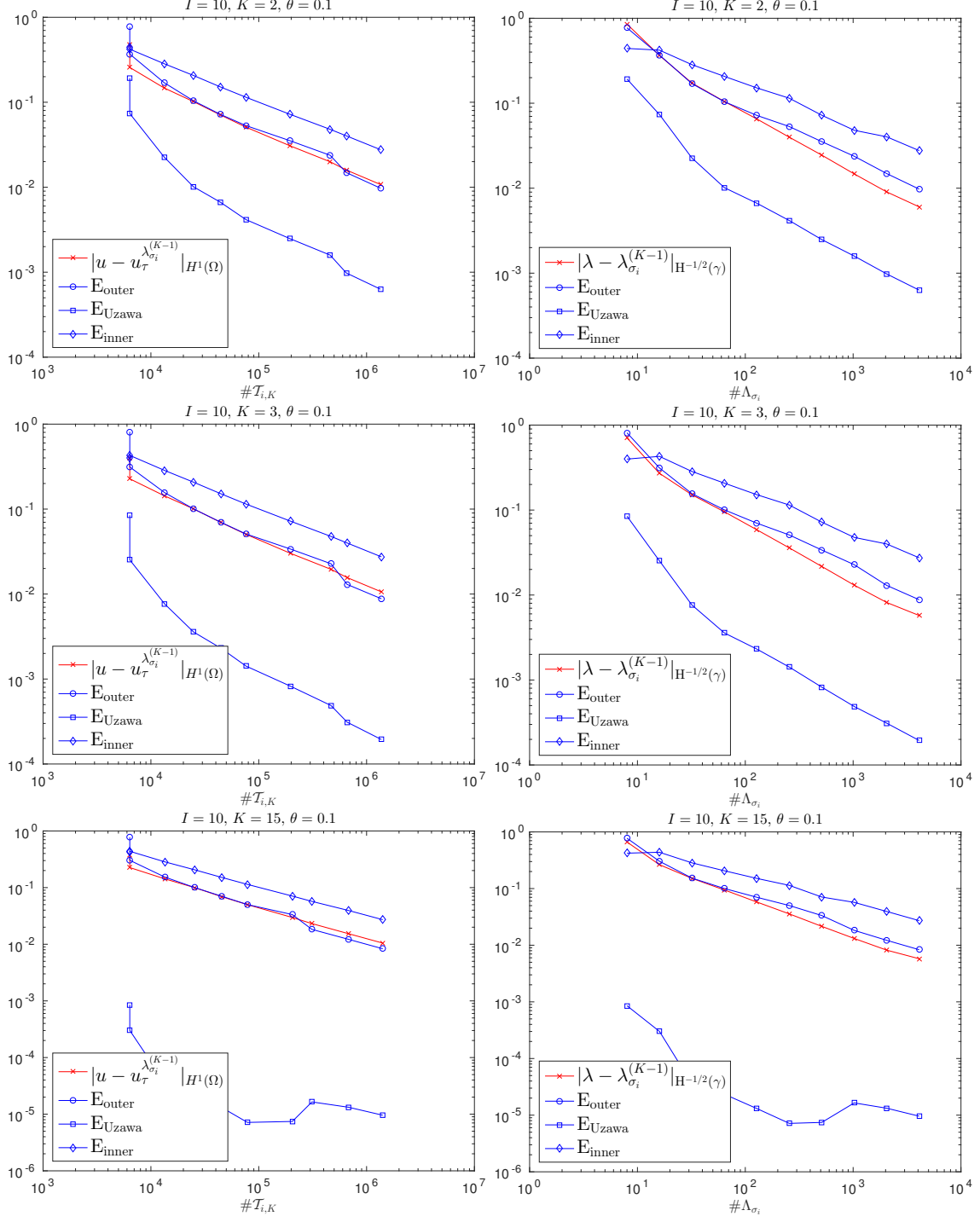
Figure 5: Errors |u - u_{\tau}^{\lambda_{\sigma_i}^{(K-1)}}|_{H^1(\Omega)} (left) and \|\lambda - \lambda_{\sigma_i}^{(K-1)}\|_{H^{-1/2}(\gamma)} (right), and estimators for \zeta = \sqrt{2} , \theta = 0.1 , and K = 2 (top), K = 3 (middle) and K = 15 (bottom).
