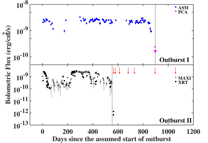
Fig. 1. Bolometric flux (0.01–100 keV) curves for outbursts I and II ( upper and lower panels , respectively). The zero points correspond to MJD 51265 for outburst I and MJD 57256 for outburst II. The vertical grey dotted lines indicate the time of the end of the respective outbursts (MJD 52162 and MJD 57809.7, respectively). For outburst I, the ASM data are shown in blue and the PCA data near the end of the outburst (including the upper limit indicated by the downward facing triangle) are shown in magenta. For outburst II, the MAXI and XRT data are shown by open and filled black circles, respectively. The vertical red arrows in the lower panel indicate the times of the observations of the source in quiescence after the end of outburst II (see Sect. 2.2 and Table 1, for details).
