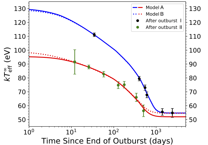
Fig. 2. kT_{\text{eff}}^{\infty} evolution of MXB 1659–29 after outbursts I and II (black and green points, respectively). We have modelled this observed evolution with the crust heating and cooling code NSCool . The modelled cooling curves after outbursts I and II are shown in blue and red, respectively. Model A (shown by the solid lines) indicates the fit when all the parameters were free to vary. Model B (shown by the dotted lines) assumes that y_{\text{light}} after both the outbursts is the same and, therefore, that the crust returns to the same observed base level. It should be noted that Models A and B have parameters that are consistent with one another within their error bands. This is shown in Fig. 3 and Table 2.
