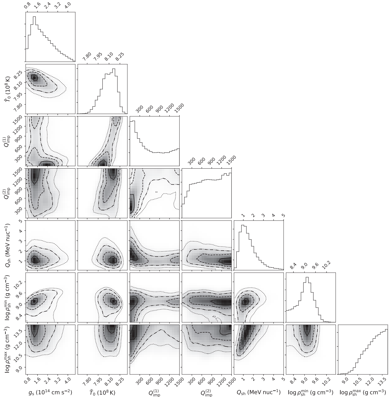
Figure 7. Results of model 2 for a selection of parameters. The solid, dashed, dashed-dotted, and dotted curves show, respectively, the 0.5\sigma , 1.0\sigma , 1.5\sigma , and 2.0\sigma levels in the 2D histograms.
