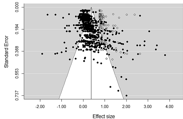
Fig. 2 Funnel plot
