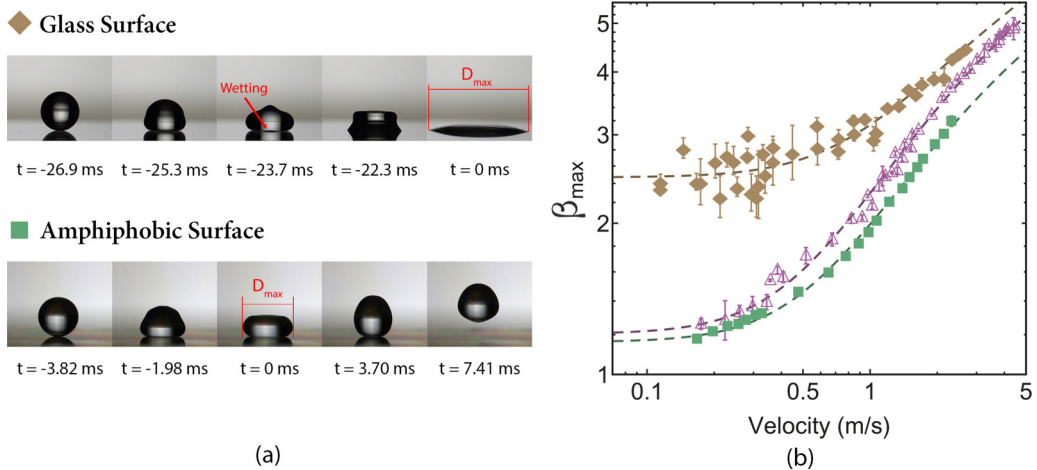
FIG. 4. (a) Water droplet impacting on hydrophilic glass (top) and an amphiphobic surface (bottom) at v_{\text{imp}} \sim 0.22 m/s. t = 0 is defined at the time when the spreading diameter is equal to D_{\max} . (b) Spreading ratio as function of impact velocity of water droplets impacting on hydrophilic glass (brown diamonds) and the amphiphobic surface (green squares) compared to the stainless steel measurements (open upward purple triangles). The dashed lines are the best fits of Eq. (2). Again, \beta_{\max} is determined within a timescale of 30 ms after impact, and the influence of long timescale wetting is currently neglected.
