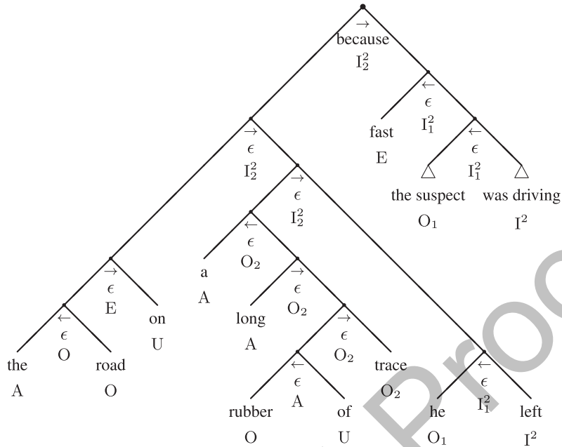
Fig. 10. The fully expanded syntactic adtree of example 1.
