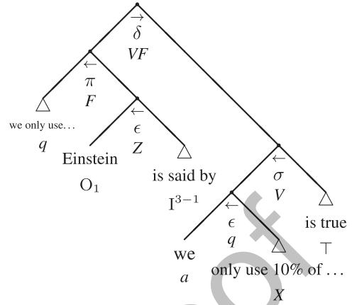
Fig. 21. The compact argumentative adtree of example 4
