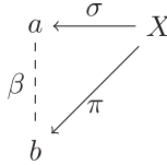
Fig. 2. Argument diagram of a first-order subject argument.
