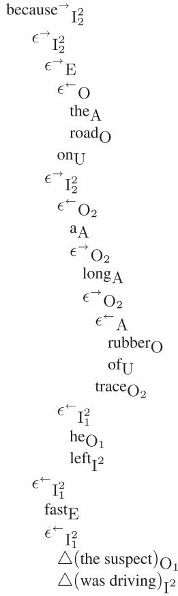
Fig. 11. The fully expanded tabular adtree of example 1.
