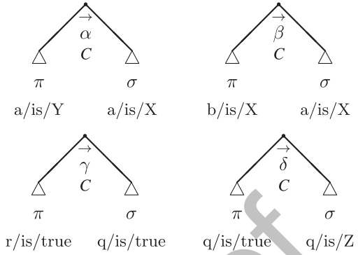
Fig. 13. The abstract arg-adtrees of arguments in the four quadrants.
