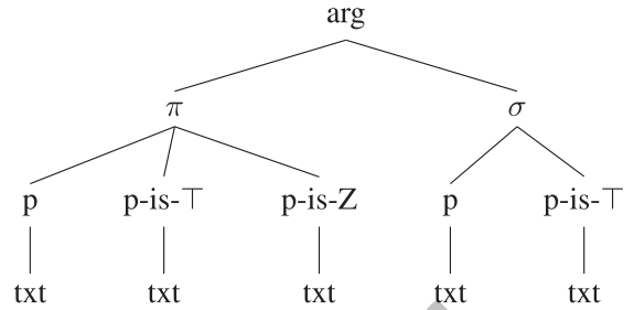
Fig. 7. Levels of abstraction within arguments.
