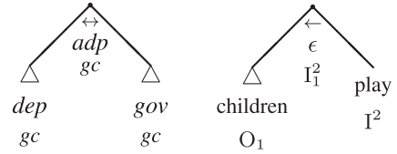
Fig. 8. The abstract adtree structure and example 0.
