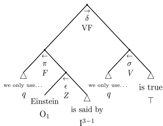
Figure 3 – The arg-adtrees of Example 4 – revisited
