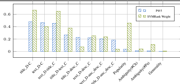
Figure 1: Feature importance: 1) P@5 of individual features, 2) weights in SVM-Rank model
