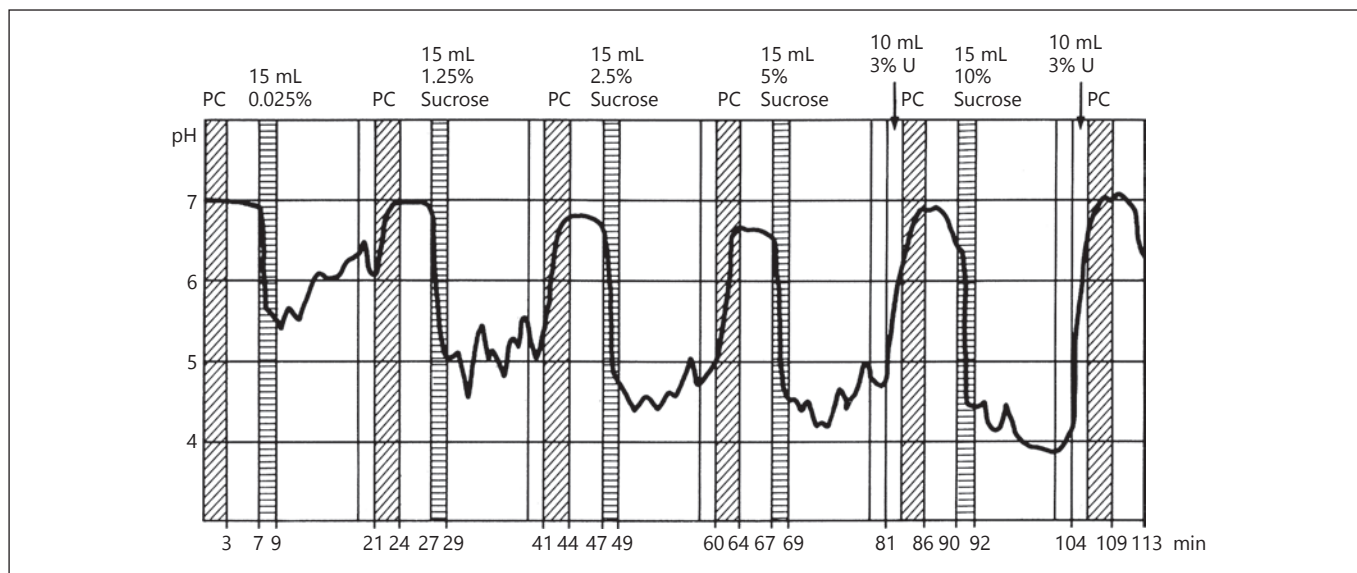
Fig. 1. pH curves in dental plaque after consecutive rinses with solutions of increasing sucrose concentrations [Imfeld, 1977].
