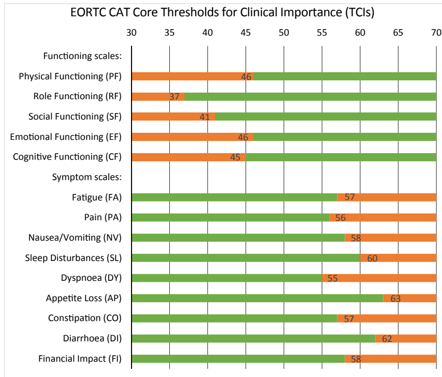
Fig. 1. Thresholds for clinical importance (TCIs) for the functioning and symptom scales of the EORTC CAT Core. TCIs are shown inside the bars. Patient scores in the orange range of the bar (i.e., equal or below the TCI for functioning scales, and equal or above the TCI for symptom scales) indicate clinically important problems or symptoms. (For interpretation of the references to color in this figure legend, the reader is referred to the Web version of this article.)
