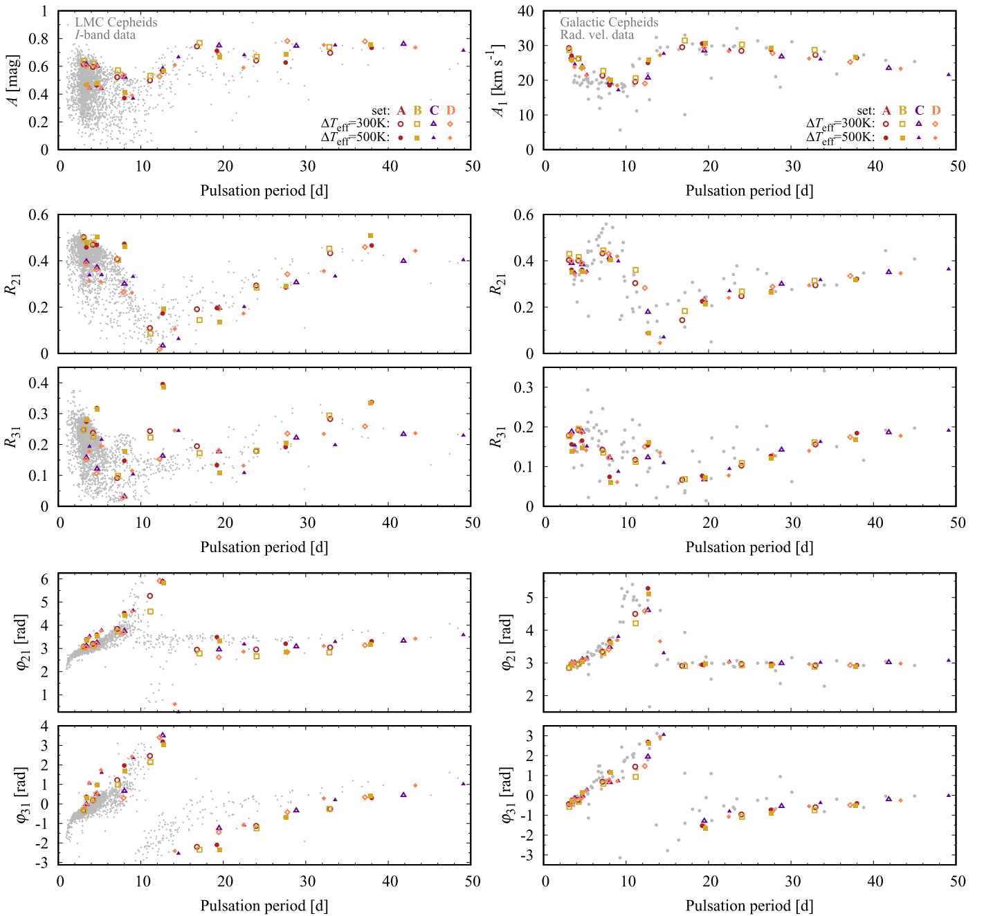
Figure 15. Amplitudes and Fourier parameters for I -band light curves (left panel) and radial velocity curves (right panel). Observations are marked with gray circles. Light-curve data are from Soszyński et al. (2015) and Ulaczyk et al. (2013), and radial velocity curve data are from Storm et al. (2011). For the light curves the peak-to-peak amplitude is shown, while for radial velocity curves the Fourier amplitude is scaled with a p -factor of 1.3. Models are plotted with colored symbols.
