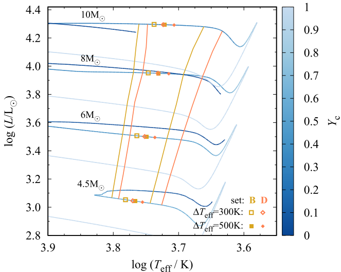
Figure 13. Evolutionary tracks in the H-R diagram, shaded to show the core He mass fraction, Y_c . Blue and red edges of the instability strip for convective sets B and D are shown, along with the locations where nonlinear Cepheid models are computed (symbols).
