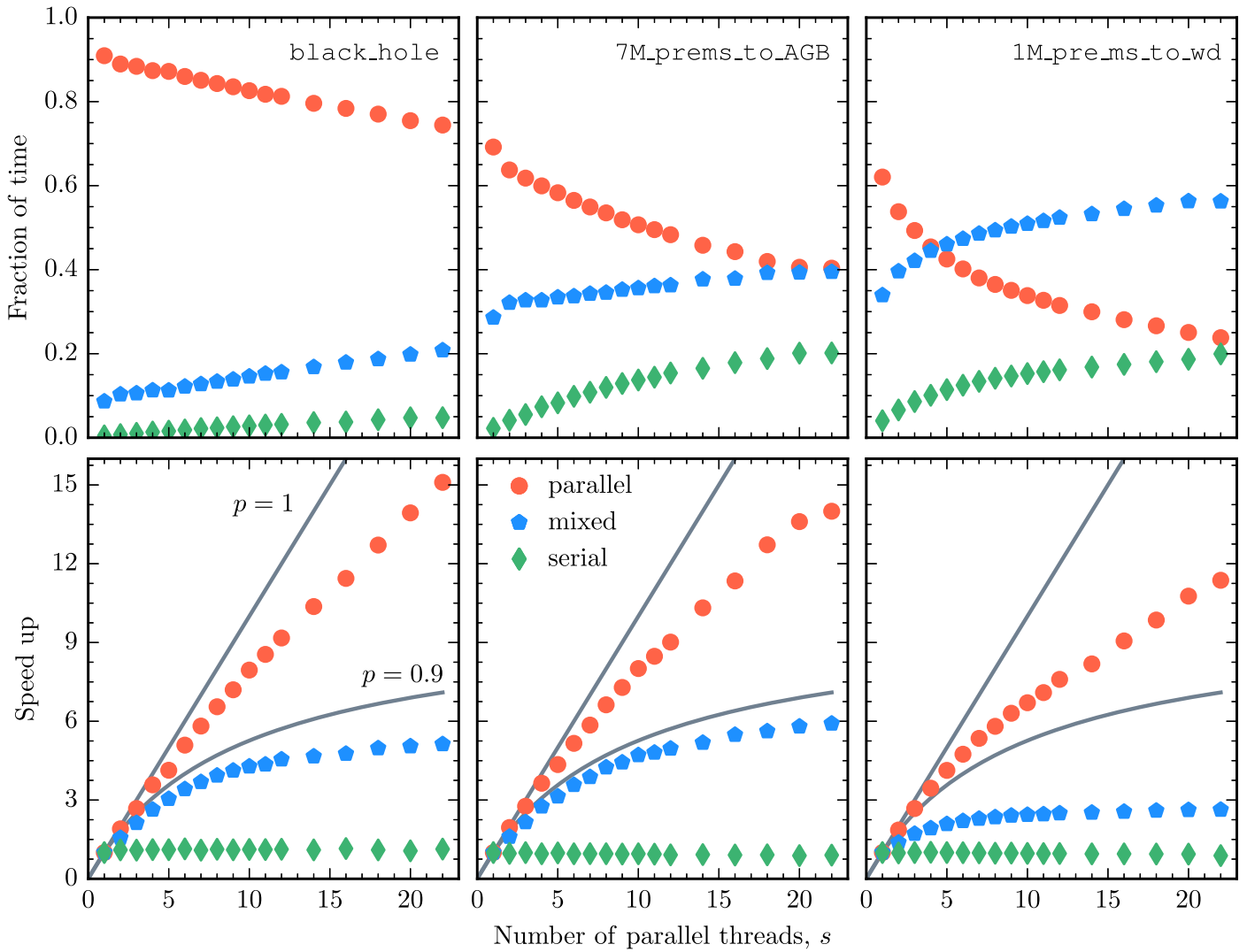
Figure 48. Breakdown of the fraction of the execution time (top row) and the speedup (bottom row) of three different categories listed in the text. Each column is a single test case. The line in the bottom panels is Equation (46) for p = 0.9 and p = 1 .
