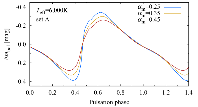
Figure 6. Bolometric light curve of the T_{\text{eff}} = 6000 K Cepheid model with convective parameters of set A but with varying eddy-viscous dissipation \alpha_m .
