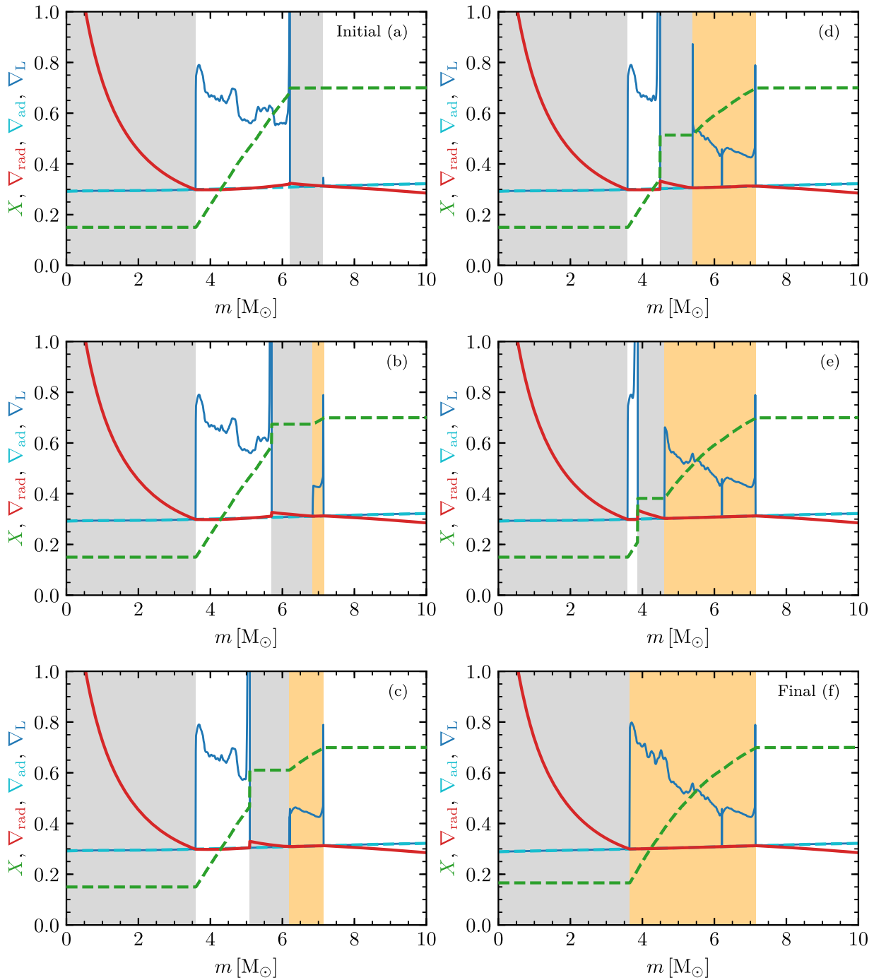
Figure 40. Profiles of \nabla_{\text{rad}} , \nabla_{\text{ad}} , \nabla_L , and X as a function of mass coordinate, in the inner part of the 16 M_{\odot} MS star at X_c = 0.15 . The panels show the outcome of an artificial switch from the predictive mixing scheme to the CPM scheme. The initial state (a) is shown in the top left panel, and the subsequent panels, running in alphabetical order (b), ..., (f), show how this state evolves during the CPM iterations. Gray (gold) shading indicates convection (semiconvection) regions.
