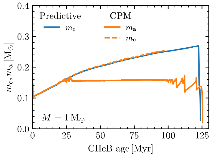
Figure 44. Mass coordinates of the convective core boundary ( m_c ) and the top of the abundance gradient region ( m_a ) as a function of CHEB age, for the 1 M_{\odot} star. Different line colors show the separate runs discussed in the text.
