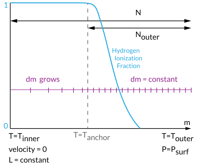
Figure 2. Grid structure in RSP. The inner boundary at the base of the static envelope is defined by a chosen temperature ( RSP\_T\_inner ). The model surface has a fixed temperature T_{\text{outer}} , derived from T_{\text{eff}} , and pressure ( RSP\_P_{\text{surf}} ). The anchor temperature ( RSP\_T\_anchor ) is usually located where H ionizes, shown by the blue curve. The envelope is divided into N Lagrangian mass cells ( RSP\_nz ). Between the anchor and the surface are N_{\text{outer}} cells ( RSP\_nz\_outer ), each with a constant mass. Between the inner boundary and the anchor the mass of each cell increases.
