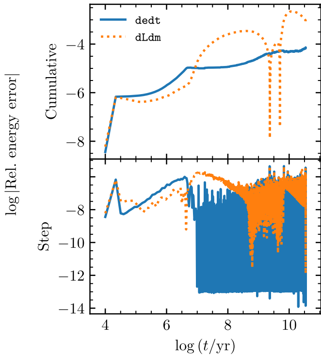
Figure 27. Comparison of energy conservation for a 0.3 M_{\odot} He WD model accreting an H/He mixture at 10^{-10} M_{\odot} \text{ yr}^{-1} . The top panel shows the relative cumulative error, and the bottom panel shows the error in each step.
