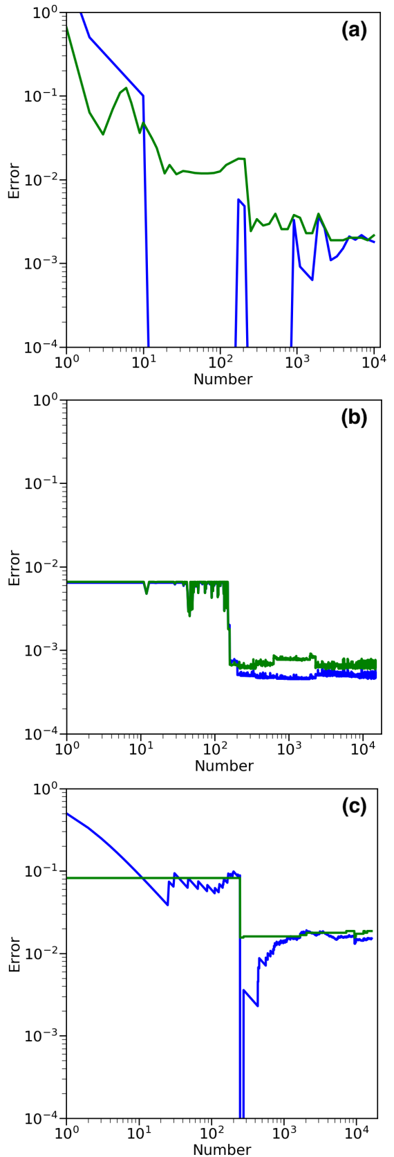
Figure 15: These panels show the learning curve, the training (blue) and validation (green) errors as a function of the number of data points in the training dataset. An optimum solution is reached when the values have tended towards similar values. (a) a simplified version for the anomaly detection strategy, (b) the logistic regression algorithm using \lambda = 0.1 , (c) the transients algorithm
