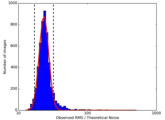
Figure 2: The rms noise is automatically measured in each image in the dataset and compared to the theoretical noise expected in the image. Here we plot a histogram of these ratios and they follow a Gaussian distribution in logarithmic space. A Gaussian distribution is fitted to the data (red line) and all images which deviate more than 2\sigma from the observed distribution (shown by the dashed black lines) are excluded from the dataset. Large deviations from this distribution typically signify calibration errors or high rms noise datasets.
