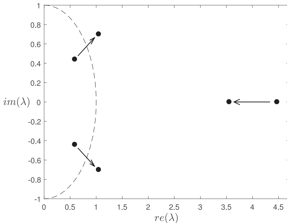
Fig. 11. Root-locus plot for model with persistence in the monetary policy rule, with \theta_\pi = 1.5 , \theta_y = 0.75 , \phi = 2 , \alpha = 0.7 , \beta = 0.99 , \xi = 0.75 , n = 0.5 , for \rho_r = 0.5, 0.7 . The Hopf bifurcation when \rho_r increases from 0.5 to 0.7 is apparent.
