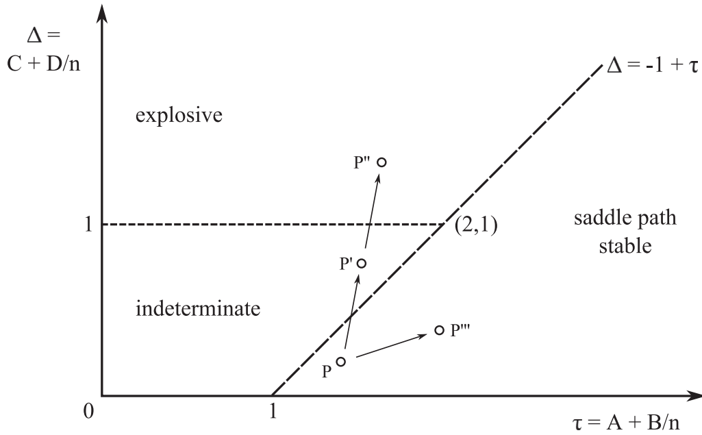
Fig. 1. Graphical illustration of Proposition 1, showing a stability plot in the trace \tau and determinant \Delta for a second order difference equation when \tau > 0 and \Delta > 0 . At point P, which lies within the saddle path stable region (i.e. it satisfies \tau - \Delta > 1 ), a decrease in n moves the model to P' or P'' if \frac{\partial \tau}{\partial(-n)} < \frac{\partial \Delta}{\partial(-n)} , or to P''' if \frac{\partial \tau}{\partial(-n)} > \frac{\partial \Delta}{\partial(-n)} . Thus a decrease in n moves the model to P' or P'' if \frac{\partial \tau}{\partial n} > \frac{\partial \Delta}{\partial n} , or to P''' if \frac{\partial \tau}{\partial n} < \frac{\partial \Delta}{\partial n} .
