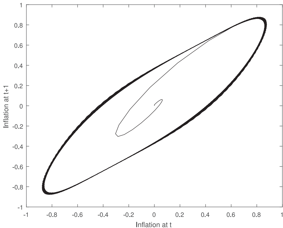
Fig. 4. Phase plot of inflation with n variable, illustrating a stable limit cycle. The parameter values are \phi = 2 , \alpha = 0.7 , \beta = 0.99 , \xi = 0.75 , \theta_\pi = 0.5 , \theta_\gamma = 4 , \mu = 1 , \Upsilon = 0 .
