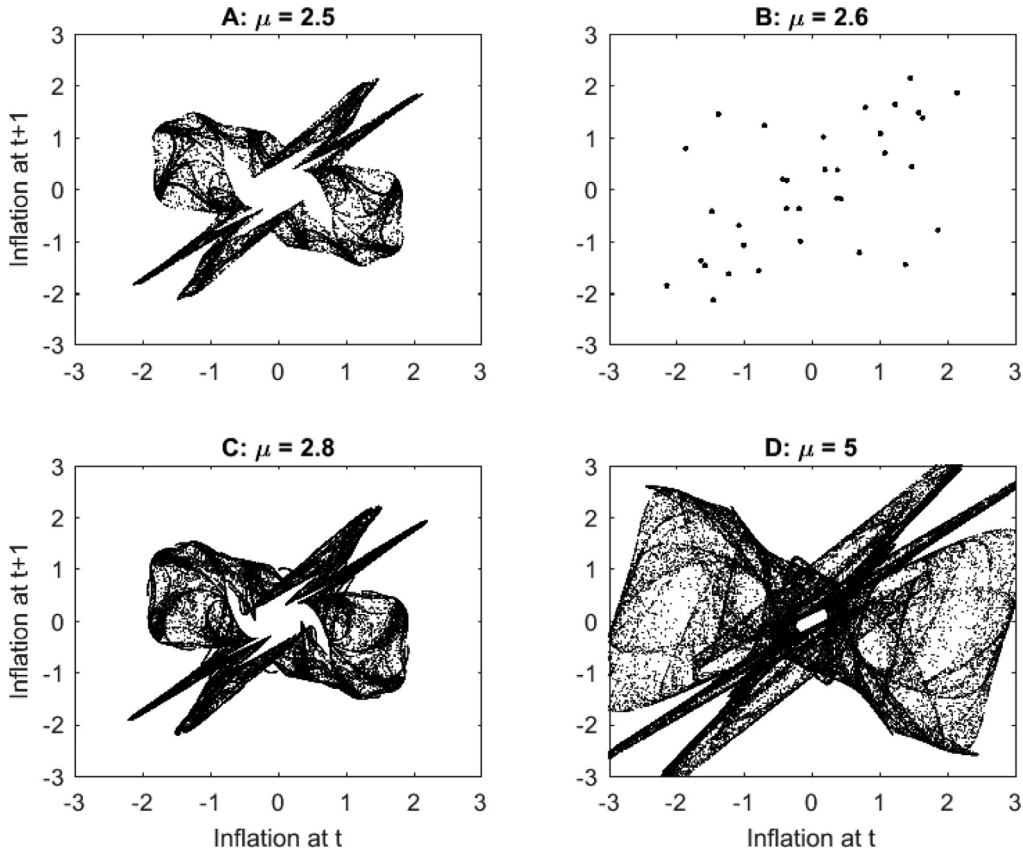
Fig. 6. Simulated trajectories for various values of \mu , illustrating the rational route to randomness . The remaining parameter values are \phi = 2 , \alpha = 0.7 , \beta = 0.99 , \xi = 0.75 , \theta_\pi = 0.3 , \theta_y = 1 , \Upsilon = 0.1 .
