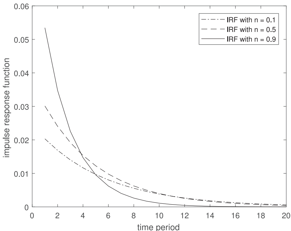
Fig. 2. Impulse response functions of inflation to a positive marginal cost shock, for the model with n fixed, for three different values of n . The remaining parameter values are \phi = 2 , \alpha = 0.7 , \beta = 0.99 , \xi = 0.75 , \theta_\pi = 1.25 , \theta_\gamma = 0.5 .
