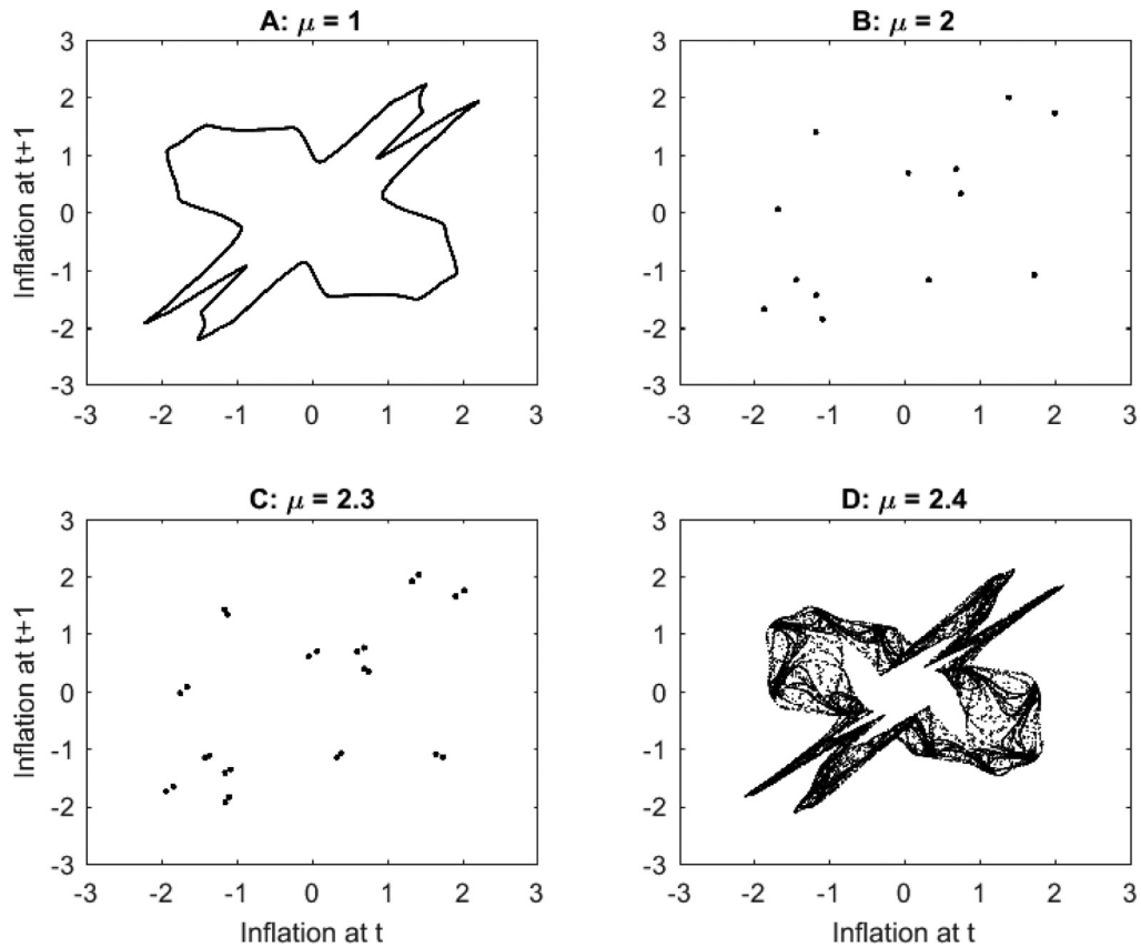
Fig. 5. Simulated trajectories for various values of \mu , illustrating the rational route to randomness. The remaining parameter values are \phi = 2 , \alpha = 0.7 , \beta = 0.99 , \xi = 0.75 , \theta_\pi = 0.3 , \theta_y = 1 , \Upsilon = 0.1 .
