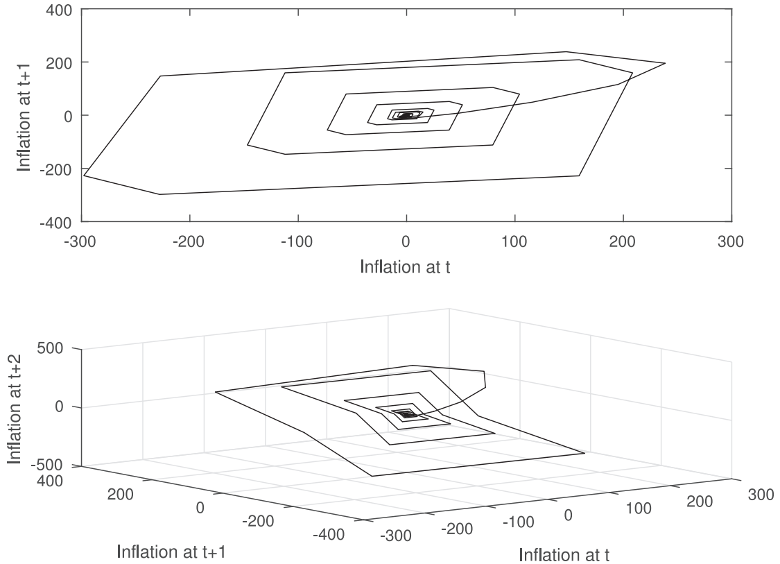
Fig. 8. Trajectories in two and three dimensions, respectively, of the first 103 iterations of the model in which \mu = 1 and \Upsilon = 0 . The remaining parameterisation is \phi = 2 , \alpha = 0.7 , \beta = 0.99 , \xi = 0.75 , \theta_\pi = 0.3 , \theta_y = 1 .
