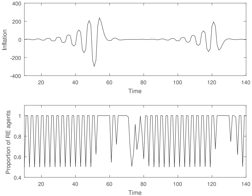
Fig. 9. Trajectories, respectively, of the first iterations 10 to 140 of the model in which \mu = 1 and \Upsilon = 0 . The remaining parameterisation is \phi = 2 , \alpha = 0.7 , \beta = 0.99 , \xi = 0.75 , \theta_\pi = 0.3 , \theta_y = 1 .
