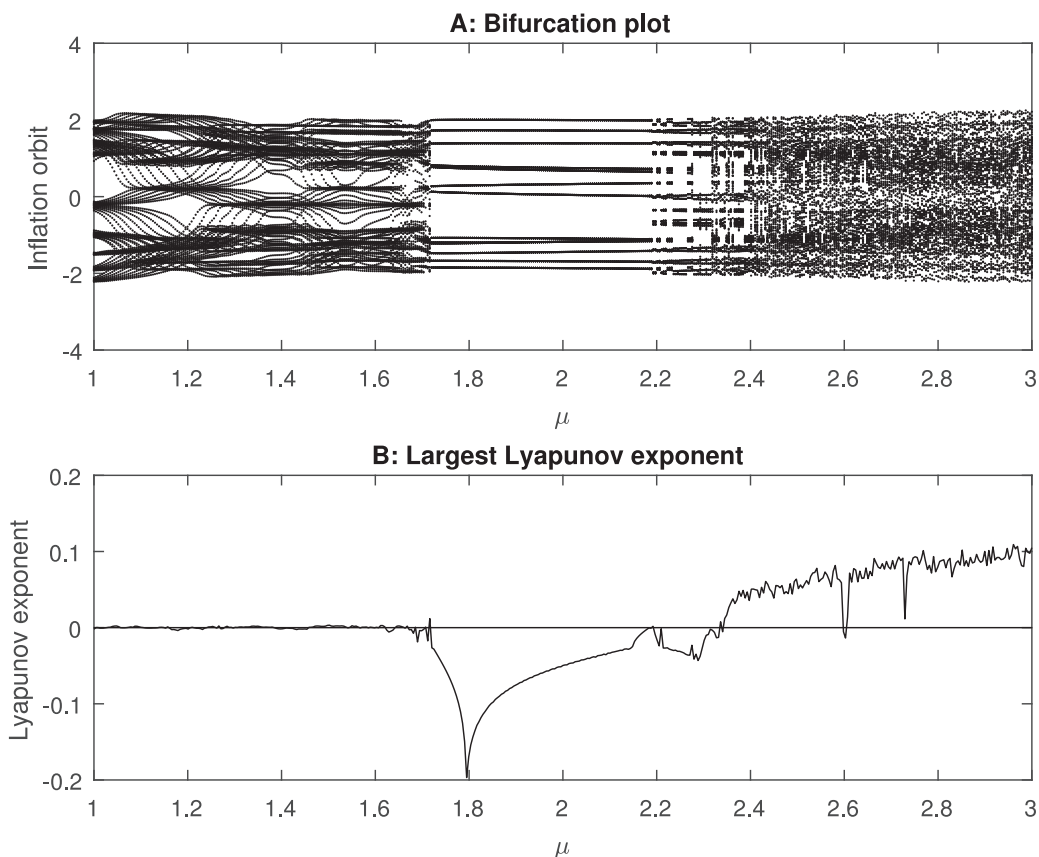
Fig. 7. Panel A: Bifurcation plot of the orbit of inflation against \mu . Panel B: Largest Lyapunov exponent against \mu . The parameter values are \phi = 2 , \alpha = 0.7 , \beta = 0.99 , \xi = 0.75 , \theta_\pi = 0.3 , \theta_y = 1 , \Upsilon = 0.1 .
