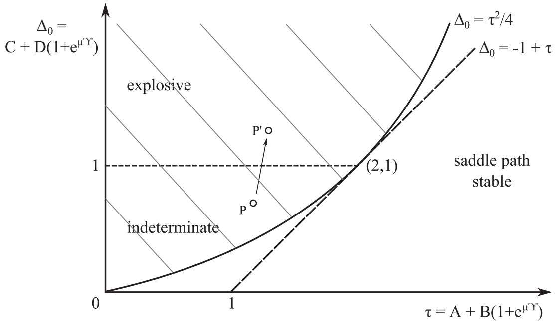
Fig. 3. Graphical illustration of Proposition 4, showing a stability plot in the trace \tau and pseudo-determinant \Delta_0 for the model in (49). Note this looks exactly the same as the stability plot in Fig. 1, as the linearised model is effectively a second order difference equation in \pi_t and z_t , but we have now shaded the region of complex conjugate eigenvalues with grey lines. As the model moves from points P to P' , as \Upsilon is increased, a Hopf bifurcation takes place.
