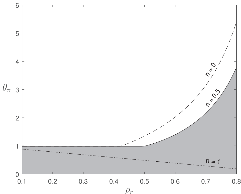
Fig. 10. Stability for model with persistence in the monetary policy rule, as a function of \theta_\pi and \rho_r , with \phi = 2 , \alpha = 0.7 , \beta = 0.99 , \xi = 0.75 , \theta_y = 0.5 , for n = 0 (dashed line), n = 0.5 (solid line), and n = 1 (dot-dashed line). (\rho_r, \theta_\pi) combinations above the constraints imply saddle path stability; the white area is saddle path stable for n = 0.5 .
