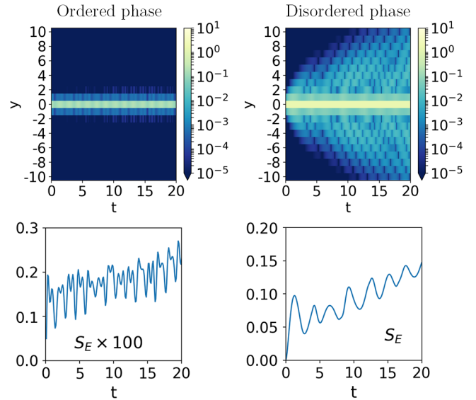
FIG. 3. (Upper panels) The time evolution of the connected correlation function, |\langle \sigma_{i+y}(x, t) \sigma_i(x, t) \rangle - \langle \sigma_{i+y}(x, t) \rangle \langle \sigma_i(x, t) \rangle| , following quenches in the 2D quantum Ising model (4) for R = 8 , J_\perp = 0 to -0.15 , and (left panels) ordered chains m = 1 and (right panels) disordered chains m = -1 . Both cases start from a J_\perp = 0 ground state. Dynamics are computed via CHAINAMPS [59]. (Lower panels) The time evolution of the entanglement entropy S_E following the same quenches. Note the y axis of the lower left panel has been increased by a factor of 100. A detailed discussion of the simulations is provided in the Supplemental Material [74].
