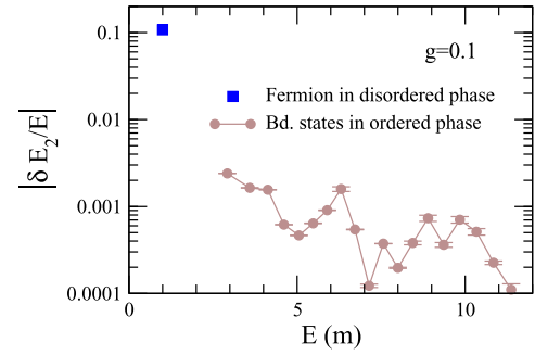
FIG. 2. We plot the relative second order correction to the energy of the first 19 zero momentum mesons ( \delta E_2/E ) coming from mixing with zero and four domain wall states in the 1D Ising field theory (2) with m = 1 and g = 0.1 . For comparison, we also plot the energy correction to the zero momentum spin flip excitation in the disordered phase. Note that the correction for the mesons is from 10^{-2} to 10^{-4} that of spin flip excitation.
