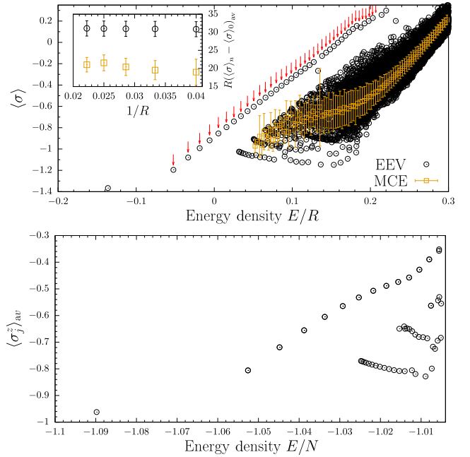
FIG. 1. (Upper panel) EEV spectrum of the spin operator \sigma(0) as a function of energy E for the 1D Ising field theory (2) with m = 1 , g = 0.1 , R = 35 . Arrows show the energies of the first 40 meson states [83]. The MCE result is shown within the continuum, with error bars denoting the standard deviation of results averaged over. (Inset) The average magnetization for the n = 11 –15 meson states compared to the MCE at the same average energy for a number of volumes R . (Lower panel) EEV spectrum of \sum_j \sigma_j^z / N as a function of energy E in the 1D lattice model (1) with J = -1 , h_x = -0.5 , h_z = 0.05 for N = 40 sites, computed with DMRG for open boundary conditions. The nonthermal states are mesonlike and confined to the vicinity of a boundary.
