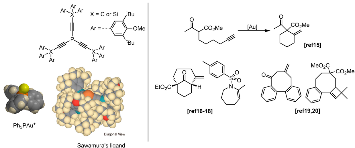
Figure 2. Left: \text{PPh}_3\text{Au}^+ and Sawamura's holey ligand ( X = \text{Si} or \text{C} ) and the corresponding space-filling model (beige = hydrogen, black = carbon, red = oxygen, cyan = silicon, orange = phosphorus and yellow = gold) for X = \text{Si} (Adapted with permission from Org. Lett. 2010 , 12 , 4380–4383. Copyright 2010 American Chemical Society). Right: various transformations to form cyclic products for which an increased reaction rate using holey phosphine was observed.
