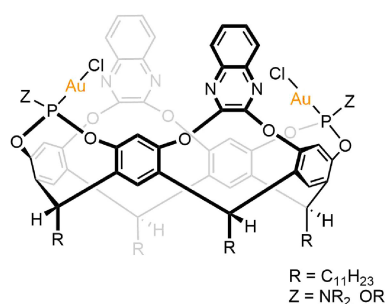
Figure 4. A dinuclear resorcin[4]arene cavitant with two gold complexes.
