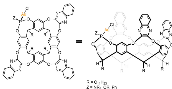
Figure 3. A resorcin[4]arene-based cavitant that functions as a ligand for the gold atom.
