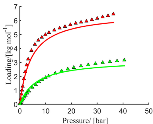
Fig. 6. Isotherms based on the parameters estimated from the breakthrough fitting (lines) and experimental adsorption isotherms measured independently (symbols) adsorption isotherms obtained for the adsorption of pure CO 2 (red) and CH 4 (green) by ITQ-29 zeolite at 298 K MSSR_{CO_2} = 0.16 [-] and MSSR_{CH_4} = 0.023 [-]. (For interpretation of the references to color in this figure legend, the reader is referred to the Web version of this article.)
