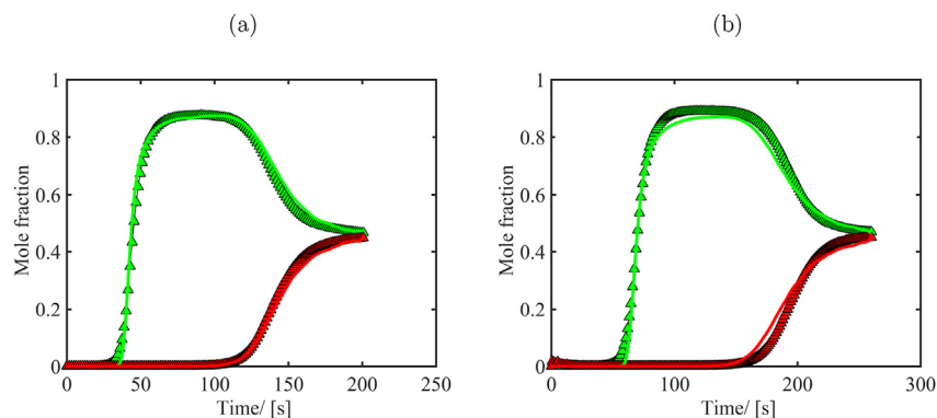
Fig. 5. Experimental breakthrough data (symbols) and theoretical breakthrough curves (lines) obtained for the optimized estimated parameter, Pe = \infty . An equimolar mixture of CO 2 (red) and CH 4 (green) is adsorbed by ITQ-29 zeolite (a) at 11 bar (b) at 16 bar and 298 K. (For interpretation of the references to color in this figure legend, the reader is referred to the Web version of this article.)
