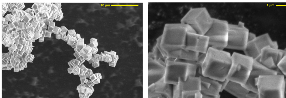
Fig. 1. SEM images of ITQ-29 zeolite used in this study.
