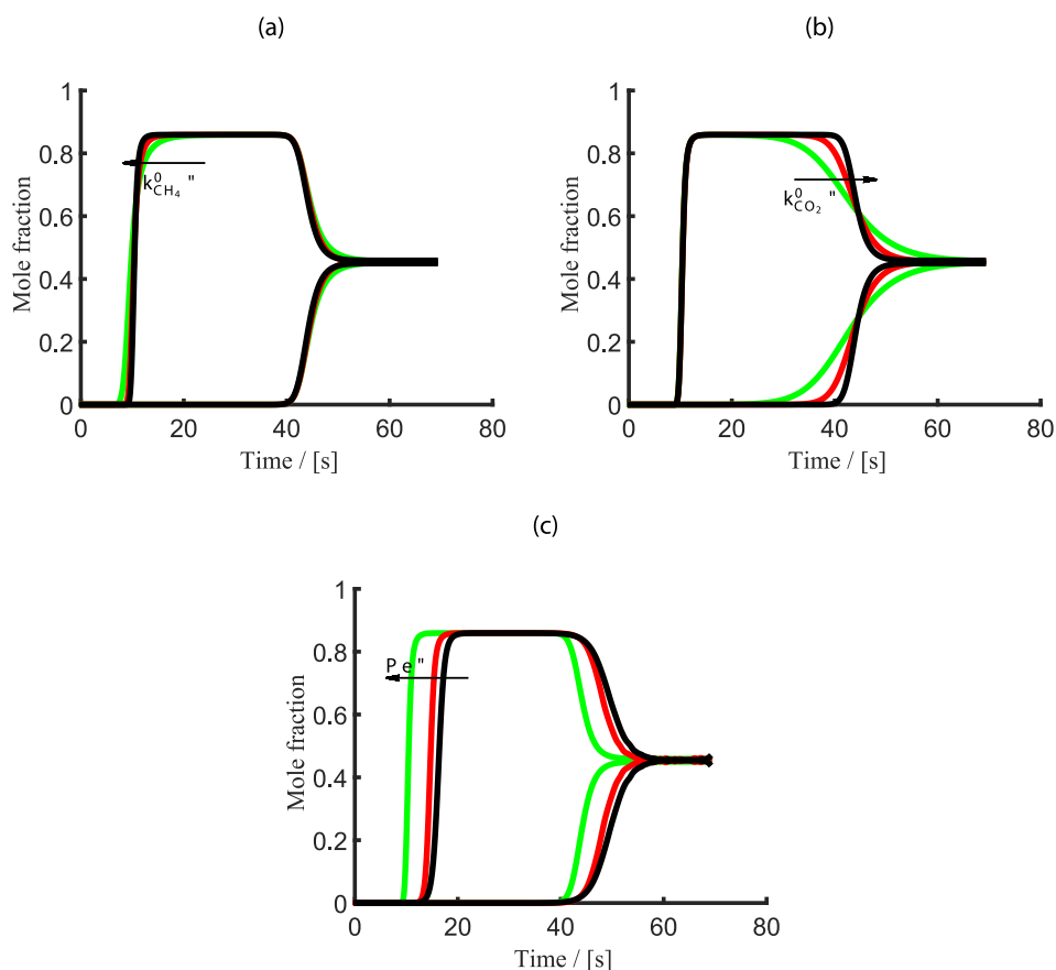
Fig. 2. Theoretical breakthrough curves obtained for different sets of mass transfer coefficient and Péclet number (a) Pe = \infty , k'_{\text{CH}_4} = 15 and k'_{\text{CH}_4} = 15 black, 7 red, 3 green (b) Pe = \infty , k'_{\text{CH}_4} = 15 and k'_{\text{CO}_2} = 15 black, 7 red, 3 green (c) k'_{\text{CO}_2} = 15 , k'_{\text{CH}_4} = 15 and Pe = 250 black, 500 red, \infty green. An equimolar mixture of \text{CO}_2 and \text{CH}_4 is adsorbed by ITQ-29 zeolite at 2 bar and 298 K. Note: the experimentally measured Henry coefficients are used in these breakthrough calculations ( K_{\text{H},\text{CO}_2}^{\text{exp}} = 1.2 [mol kg -1 bar -1 ], K_{\text{H},\text{CH}_4}^{\text{exp}} = 0.3 [mol kg -1 bar -1 ]). (For interpretation of the references to color in this figure legend, the reader is referred to the Web version of this article.)
