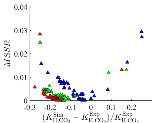
Fig. 3. Distribution of values of MSSR as a function of obtained Henry coefficients for \text{CO}_2 for different fixed values of Péclet number Pe = \infty (blue), Pe = 500 (green) and Pe = 250 (red). Fitted Henry coefficients are obtained by fitting the theoretical breakthrough curves to the experimental breakthrough curves. An equimolar mixture of \text{CO}_2 and \text{CH}_4 is adsorbed by ITQ-29 zeolite at 2 bar and 298 K. The values for Henry coefficients obtained from the experiments are shown in SI. (For interpretation of the references to color in this figure legend, the reader is referred to the Web version of this article.)
