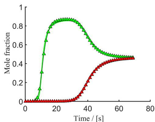
Fig. 4. Experimental breakthrough data (symbols) and theoretical breakthrough curves (lines) obtained for the optimized estimated parameter, Pe = \infty . An equimolar mixture of \text{CO}_2 (red) and \text{CH}_4 (green) is adsorbed by ITQ-29 zeolite at 2 bar and 298 K. (For interpretation of the references to color in this figure legend, the reader is referred to the Web version of this article.)
