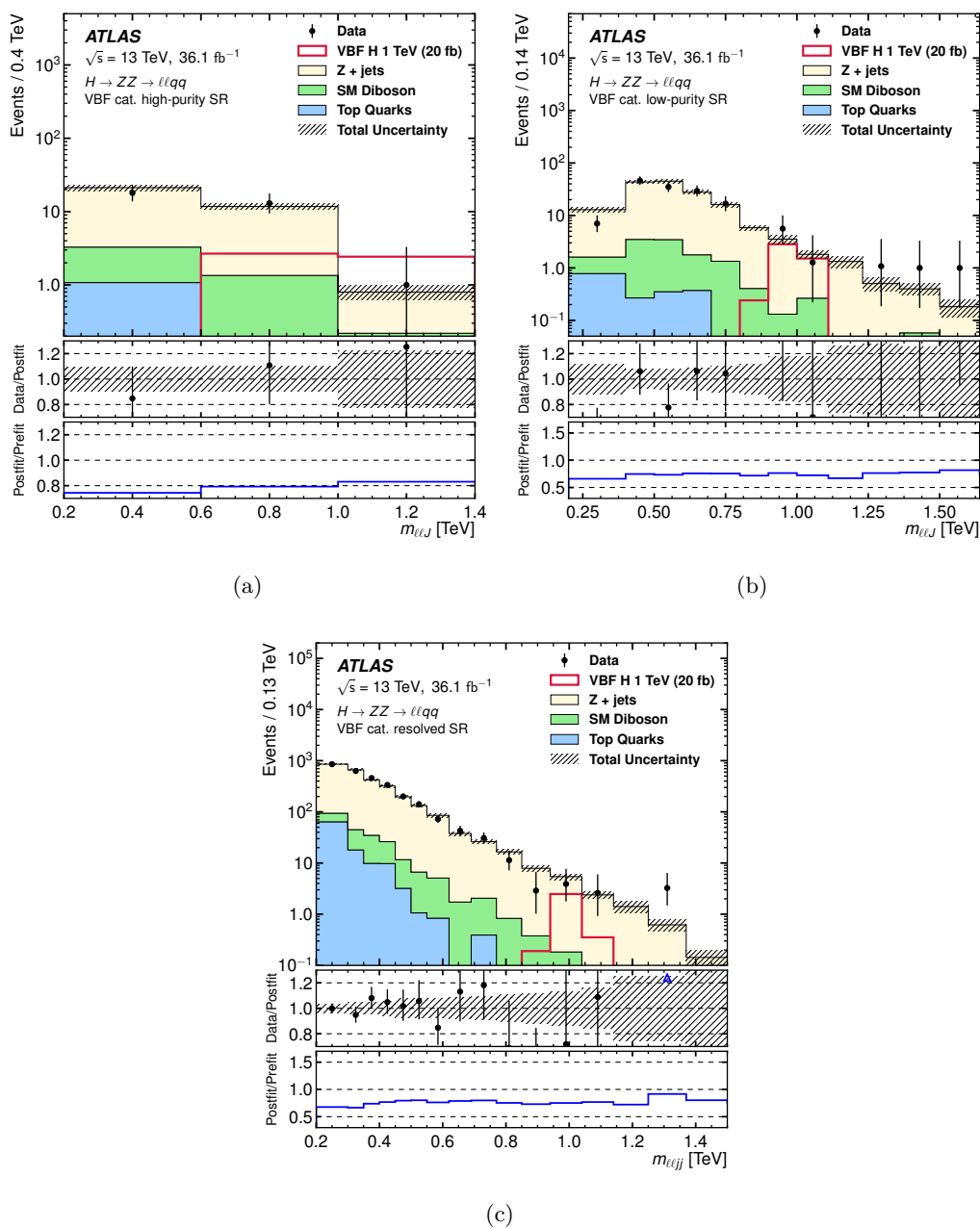
Figure 7. Comparisons of the observed data and expected background distributions of the final discriminants of the VBF category for the H \rightarrow ZZ \rightarrow \ell\ell q\bar{q} search: m_{\ell\ell J} of (a) high-purity and (b) low-purity signal regions; (c) m_{\ell\ell jj} of the resolved signal region. For illustration, expected distributions from the VBF production of a 1 TeV Higgs boson with \sigma \times \mathcal{B}(H \rightarrow ZZ) = 20 fb are also shown. The middle panes show the ratios of the observed data to the background predictions. The uncertainty in the total background prediction, shown as bands, combines statistical and systematic contributions. The blue triangles in the middle panes indicate bins where the ratio is nonzero and outside the vertical range of the plot. The bottom panes show the ratios of the post-fit and pre-fit background predictions.
