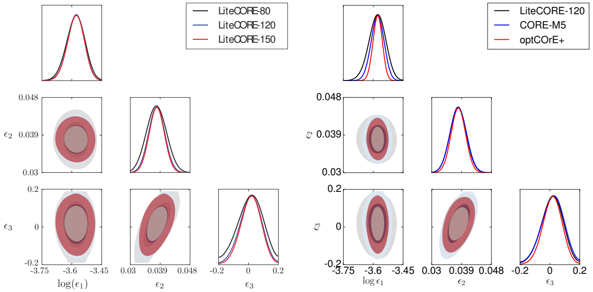
Figure 13: Compared forecasts on the Hubble flow parameters (1D and 2D marginalized posterior distributions after CMBxMCMC delensing) when the fiducial model is SL.
