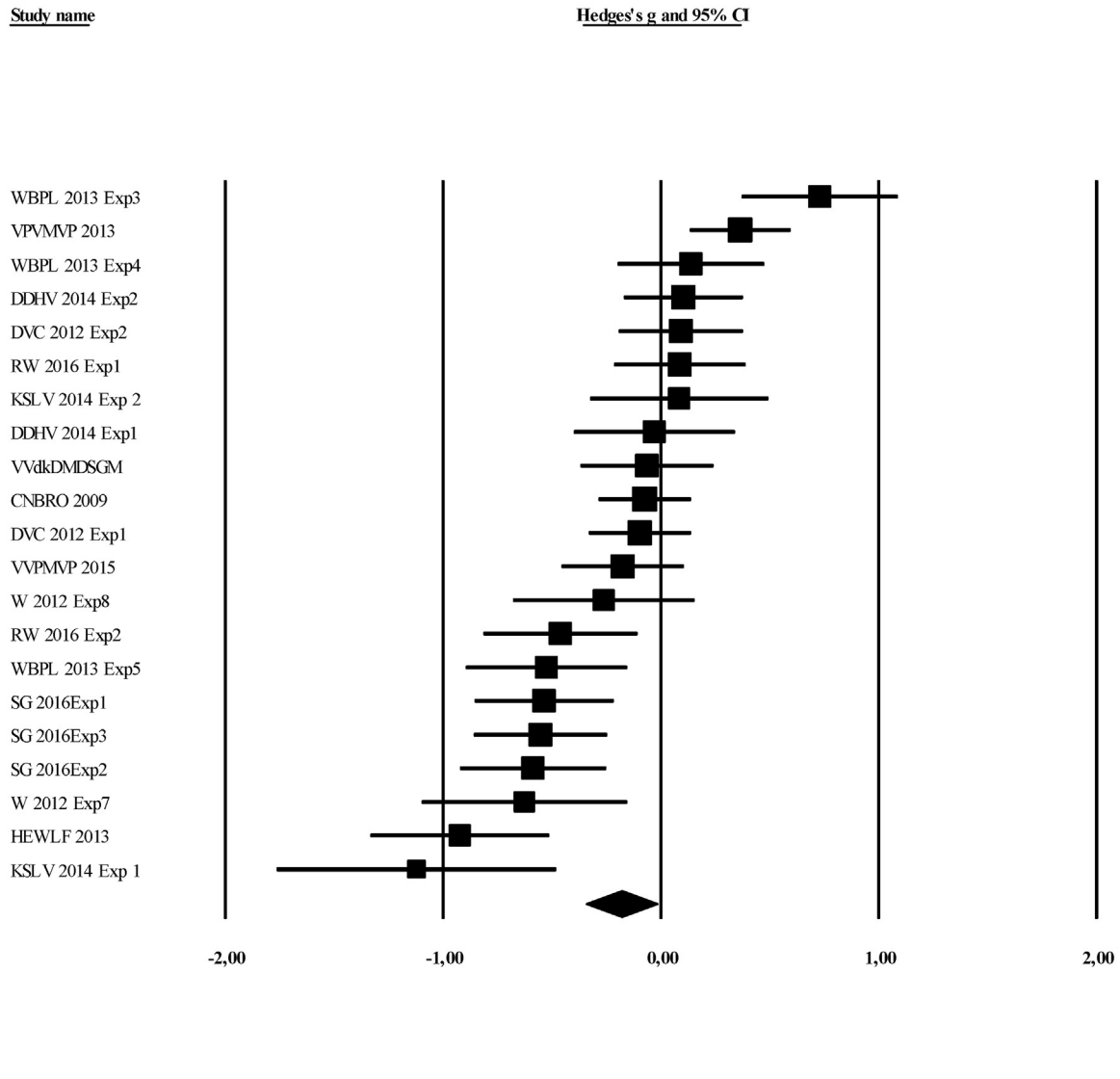
Figure 1. Forrest plot, random-effects model.
