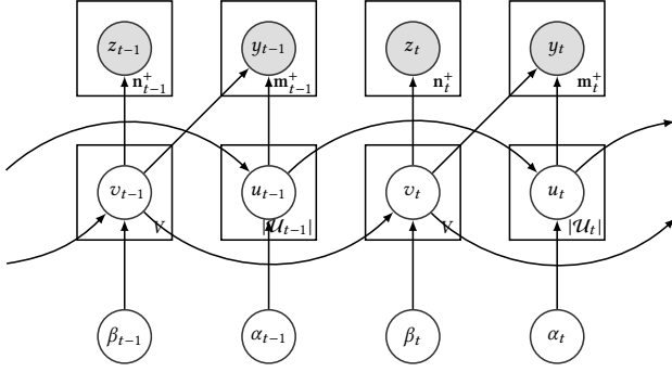
Figure 1: Graphical representation of our DUWE. Shaded nodes represent observed variables.
