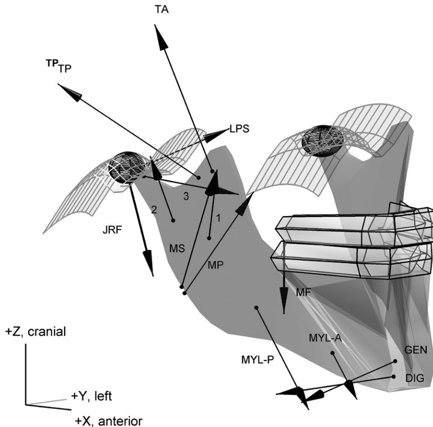
FIGURE 3 Graphical representation of the biomechanical model of the human masticatory system. Right anterior view. Arrows indicate forces (right side only). Anterior slope angle of the articular eminence (ASA). Working line of the jaw closers. More forward inclination (+15) depicted only for anterior aspect of temporalis muscle (TA). TP, posterior temporalis; MP, medial pterygoid; MA, masseter (three parts); JRF, joint reaction force; C, mandibular condyle; E, articular eminence
