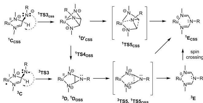
Scheme 6. Calculated reaction pathways for the conversion of intermediates 1 C CSS or 3 C to the final product 1 E CSS .
