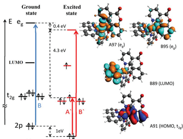
Fig. 4 Energy level diagram and some important molecular orbitals which are relevant to explain the transient Ir L 3 XANES spectra.
