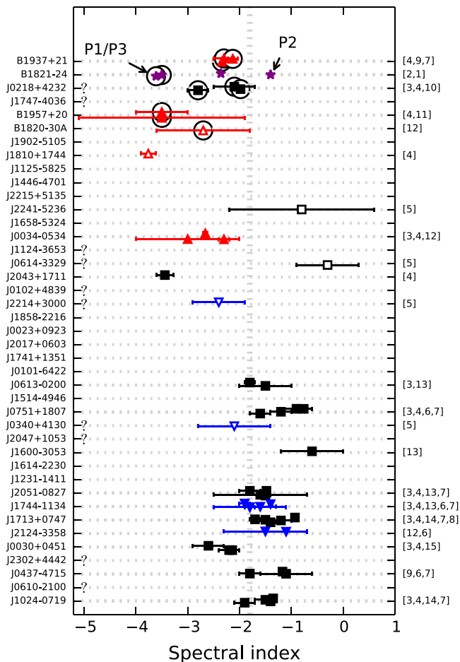
Figure 8. All available spectral indices for the radio emission of MSPs in the second Fermi catalog. Pulsars are sorted by descending values of B_{LC} . The markers follow the same scheme as in Figure 7. A small random vertical jitter was added to the markers to facilitate the visual examination of the data. A vertical line marks both the mean and the median values of the distribution of MSP spectral indices from Kramer et al. (1998). For M28A, both the spectral index of phase-averaged emission and the indices from individual components are shown. Note that component P2, the one misaligned with the \gamma -ray components, has a shallower spectrum, which is in line with Class I/III pulsars, whereas components P1/P3 have more steep spectra and are roughly aligned with the \gamma -ray emission. References: (1) this work; (2) PDR14; (3) Kuzmin & Losovsky (2001); (4) T. E. Hassall et al. 2015, in preparation; (5) Espinoza et al. (2013); (6) Kramer et al. (1998); (7) Kramer et al. (1999); (8) Kijak et al. (1998); (9) Yan et al. (2011b); (10) Navarro et al. (1995); (11) Fruchter et al. (1990); (12) Toscano et al. (1998); (13) Ord et al. (2004); (14) Xilouris et al. (1998); (15) Lommen et al. (2000).
