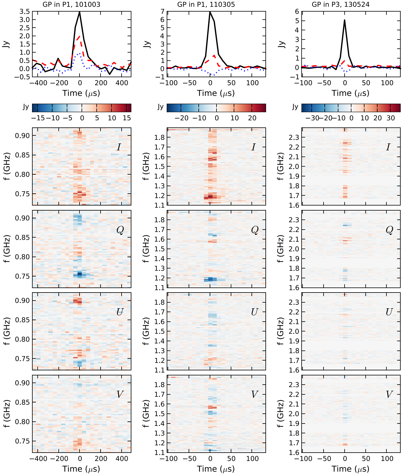
Figure 4. Examples of GRPs from the three observed bands in four Stokes components. The phase window of arrival (trailing edge of component P1 or P3) is labeled on top together with the observing date in yyymmdd format. The top row features band-integrated emission, with total intensity I (solid black line), linear polarization \sqrt{Q^2 + U^2} (red dashed line), and circular polarization V (dotted blue line). The rest of each column shows the spectra of GRPs from the top row in each of the four Stokes components. The GRPs are mostly unresolved in time and have exponential scattering tails at lower frequencies (at the bottom of the UHF and L-band observation). Note that both the time and frequency resolutions of the UHF data are four times lower than in L and S bands. The decorrelation bandwidth of scintillation due to multipath propagation in the ISM is much smaller than the width of the frequency channels. Thus, the observed frequency structure is an intrinsic property of M28A's GRPs. The polarization was corrected for Faraday rotation from the ISM and Earth's ionosphere (see Section 2.3). Within the GRPs, the position angle of linear polarization and the sign of circular polarization vary from patch to patch. Therefore, band-integrated GRPs have a smaller degree of linear and/or circular polarization.
