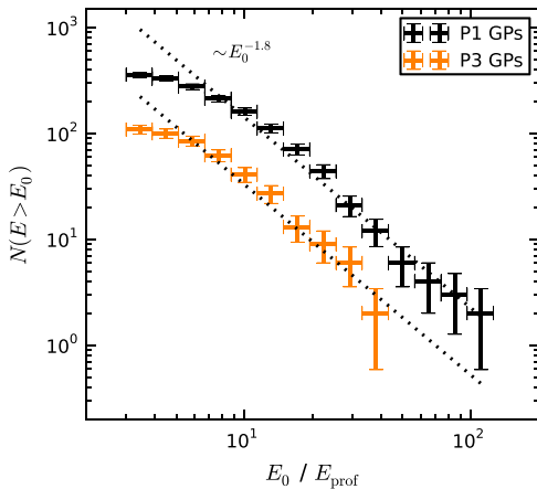
Figure 3. Cumulative energy distributions for GRPs coming from the trailing edges of components P1 and P3 in all three observing bands. The error bars correspond to the \sqrt{N} Poisson uncertainties and do not account for the under-representation of low-energy GRPs in our sample. The low-energy end of distribution is affected by a number of selection effects, described in the text.
