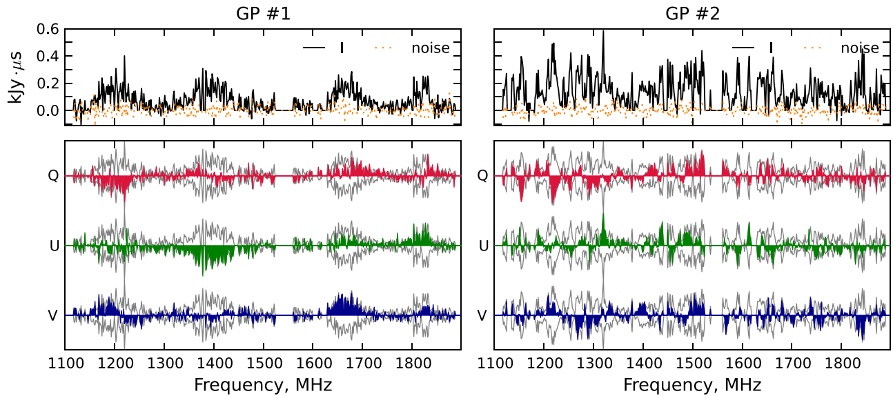
Figure 5. Spectra of two P1 GRPs recorded 20 minutes apart from each other. Top: the total intensity of GRP I(\nu) (black line) and the level of noise outside the pulse (orange dots). The signal in some of the channels was set to zero because of RFI. Bottom: the three other components of the Stokes vector for the same pulses. I(\nu) and -I(\nu) are plotted in gray together with each polarized component for reference. The GRP on the left shows visible \sim 100 MHz clumps with polarization being constant or changing slowly within each clump. The GRP on the right has a more complex frequency structure, presumably consisting of \approx 10 MHz clumps with similar polarization behavior.
