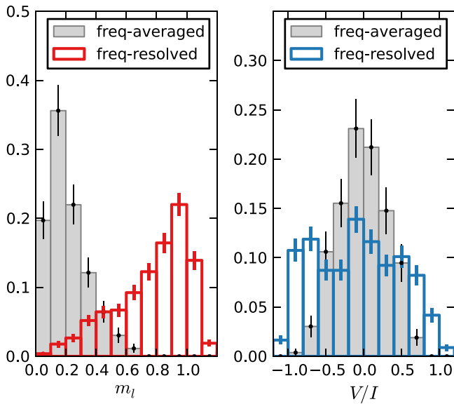
Figure 6. Fractional polarization of GRPs: linear (left) and circular (right). Filled bars show the band-integrated fractional polarization for all GRPs with S/N > 15 . Open bars show the polarization per 1.56 MHz frequency channel for all channels where the S/N of the total intensity signal was > 15 . Histograms are normalized by the sum of bar heights, and Poisson errors are shown on top of each bar. Apparent fractional polarization with magnitude above 100% is due to the influence of noise (see text for details). Individual GRP patches tend to be more polarized, but the PA varies from patch to patch, which causes gradual washing out of the polarization across the band. Depending on the intrinsic GRP width (which is unresolved in our single-pulse data), the presented polarization measurements may be biased by small-number statistics and thus may not reflect the intrinsic polarization properties of the GRP emission mechanism (see text for details).
