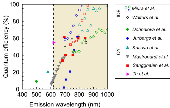
Figure 1.1: Emission efficiency of Si-QDs. Overview of the quantum yield (QY) (filled symbols) and internal quantum efficiency (IQE) (open symbols) of values found in literature for different types of Si-QDs (black symbols). IQEs from Miura et al. [8] and Walters et al. [9] and QYs from Dohnalova et al. [2], Jurbergs et al. [10], Kusova et al. [11], Mastronardi et al. [12], Sangghaleh et al. [13] and Tu et al. [14]. The shaded area indicates the emission wavelength range for which high QYs and IQE have been reported.
