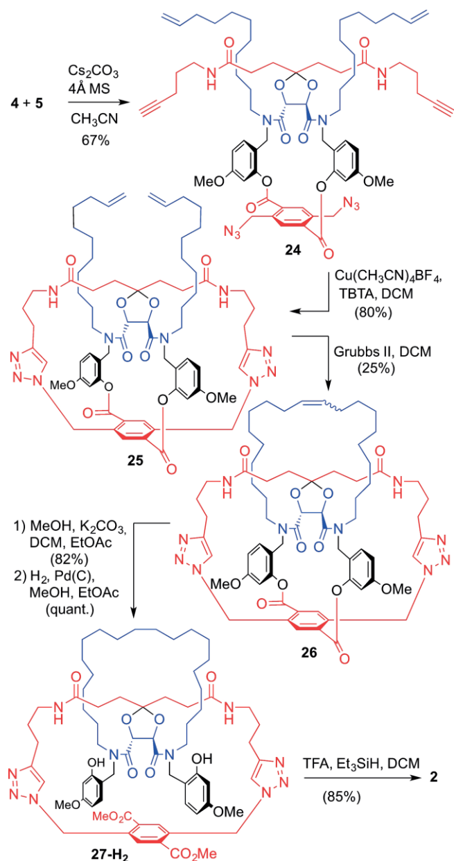
Scheme 7. End game towards quasi[1]catenane 2 .
