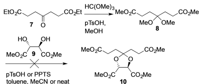
Scheme 3. Attempted synthesis of central L-(+)-tartaric acid-based core.
