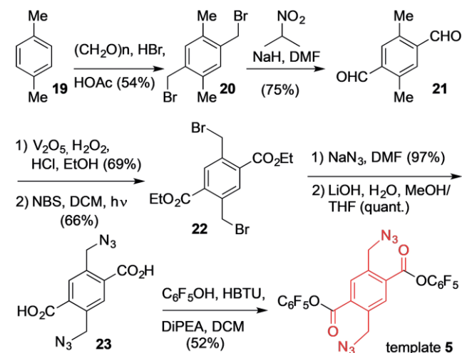
Scheme 6. Scaffold synthesis.
