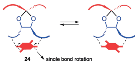
Scheme 8. Possible diastereomer formation due to hindered rotation at the terephthalic single bond ester connections.
