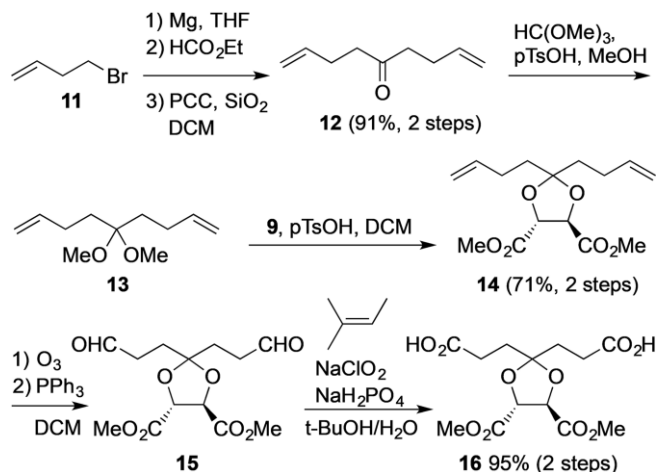
Scheme 4. Synthetic scheme of the L-(+)-tartaric acid based central core.
