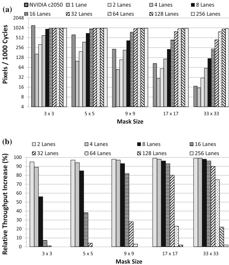
Fig. 13 Throughput, Input Size = 128 \times 128 , LS BW = 256 Bytes/Cycle. a Throughput, b Relative performance improvement (in %)
