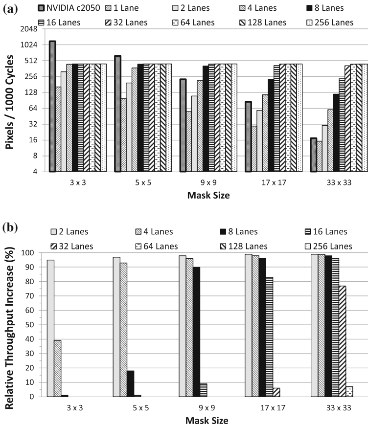
Fig. 9 Throughput, Input size = 128 \times 128 , LS BW = 16 Bytes/Cycle. a Throughput, b Relative performance improvement (in %)
