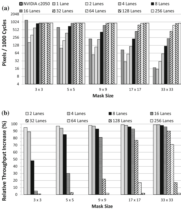
Fig. 11 Throughput, Input size = 128 \times 128 , LS BW = 64 Bytes/Cycle. a Throughput, b Relative performance improvement (in %)
