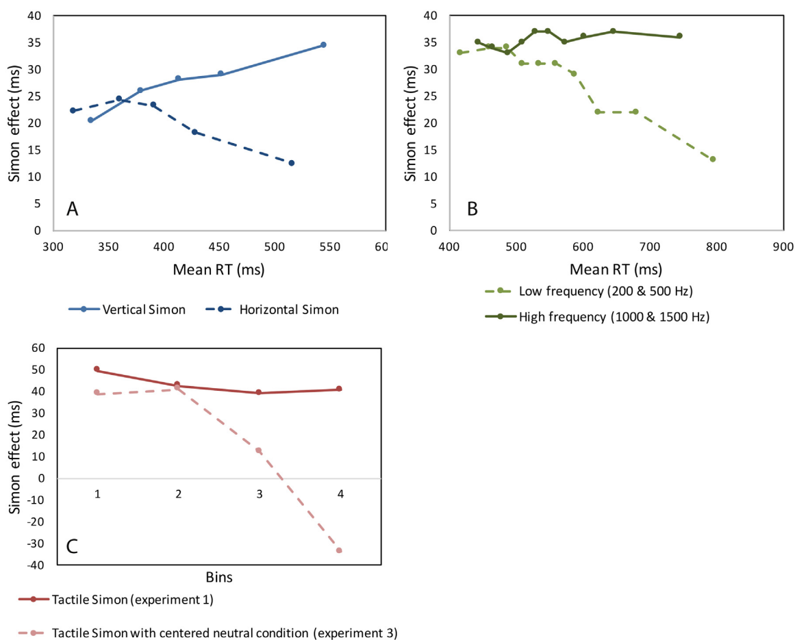
Fig. 1. Distribution of mean Simon effect, also known as delta plots, for (A) horizontal and vertical visual Simon task (data adapted with permission from Töbel et al., 2014), (B) high- and low-frequency auditory Simon task (data adapted with permission from Xiong and Proctor, 2016), and (C) tactile Simon task with- and without-central neutral condition (data adapted with permission from Salzer et al., 2014).
