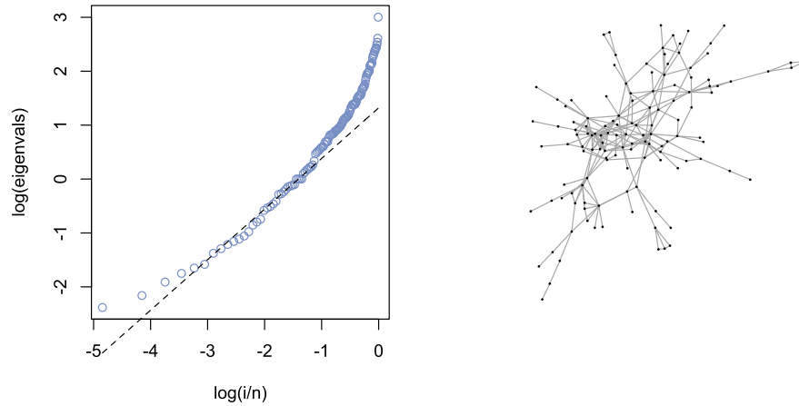
FIG 3. Plot of \log \lambda_i against \log(i/n) for the Protein interaction graph in the right panel. Fitted line has slope 0.94, corresponding to r = 2.1 in the geometry assumption.
