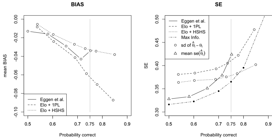
Figure 10: Bias and standard error for different computer adaptive methods at different values of the expected probability correct.
