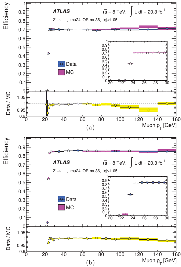
Figure 7.15: Efficiency of passing the logical OR between the two single muon triggers used in the lep-had channel for both the barrel (a) and the endcap (b) regions, for both both data (dots) and MC simulation (bands). The error bars include both statistical and systematic uncertainties. Figure taken from [241].
