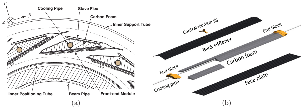
Figure 2.6: Cross section of the IBL Layout (a) and schematic representation of the composition of a stave (b).
