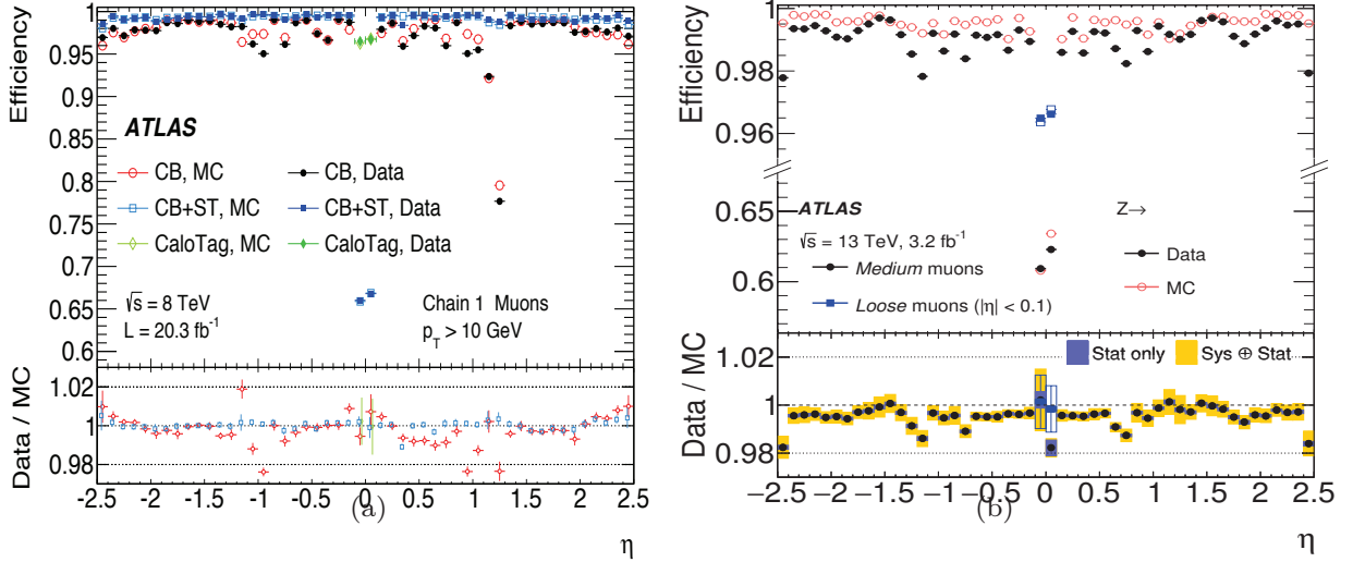
Figure 3.8: Measured muon reconstruction efficiency as a function of \eta for different type of muons reconstructed using the Chain 1 algorithm in 2012 (left) and for Loose and Medium muons selected by the Chain 3 algorithm in 2015. The figures for Run-1 and Run-2 are taken from [145] and [137], respectively.
