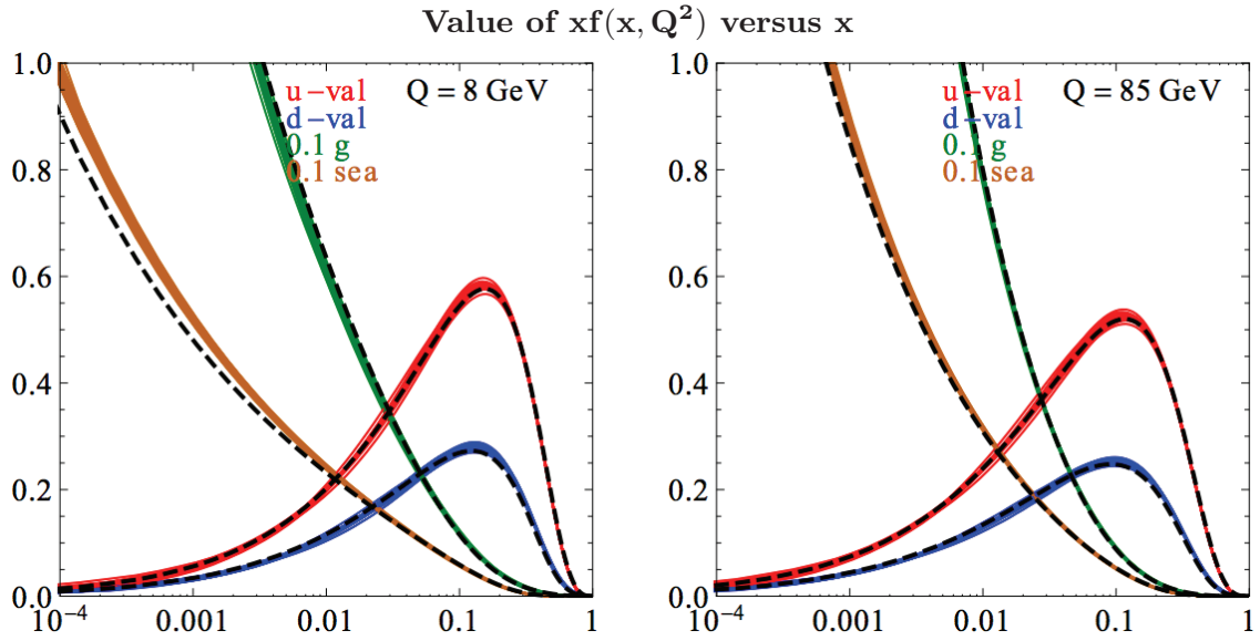
Figure 1.2: The distribution of xf(x, Q^2) for the CT10NNLO parton distribution function at two different interaction scales, for valence quarks, sea quarks and gluons. The coloured bands show the systematic uncertainties.[68].
