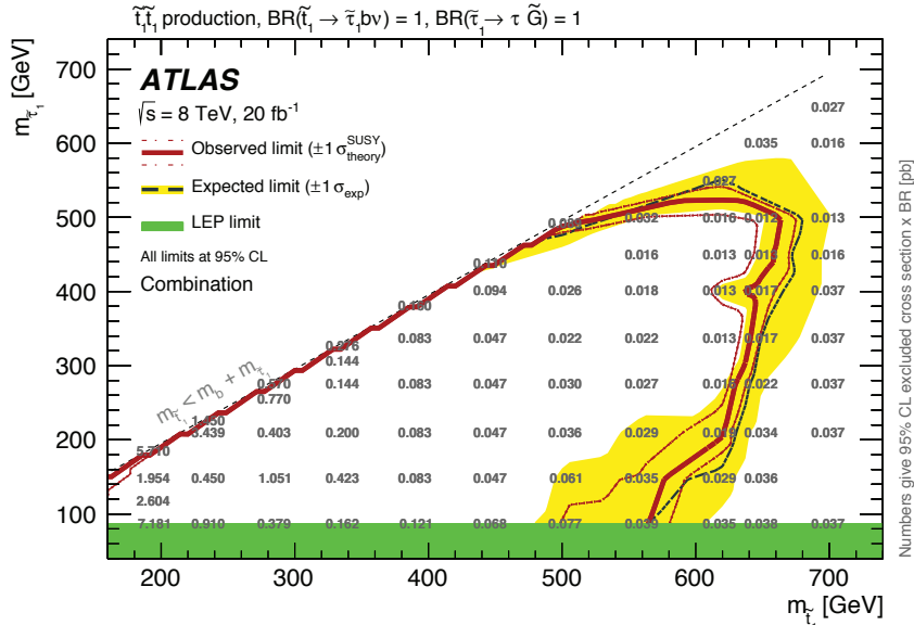
Figure S.3: Exclusion limits on the top squark production with direct decay \tilde{t}_1 \rightarrow \tilde{\tau}_1 b \nu_\tau and \tilde{\tau} \rightarrow \tau \tilde{G} at \sqrt{s} = 8 TeV. The limits on the \tilde{t} \rightarrow \tilde{\tau} production cross section in pb are reported for each signal hypothesis.
