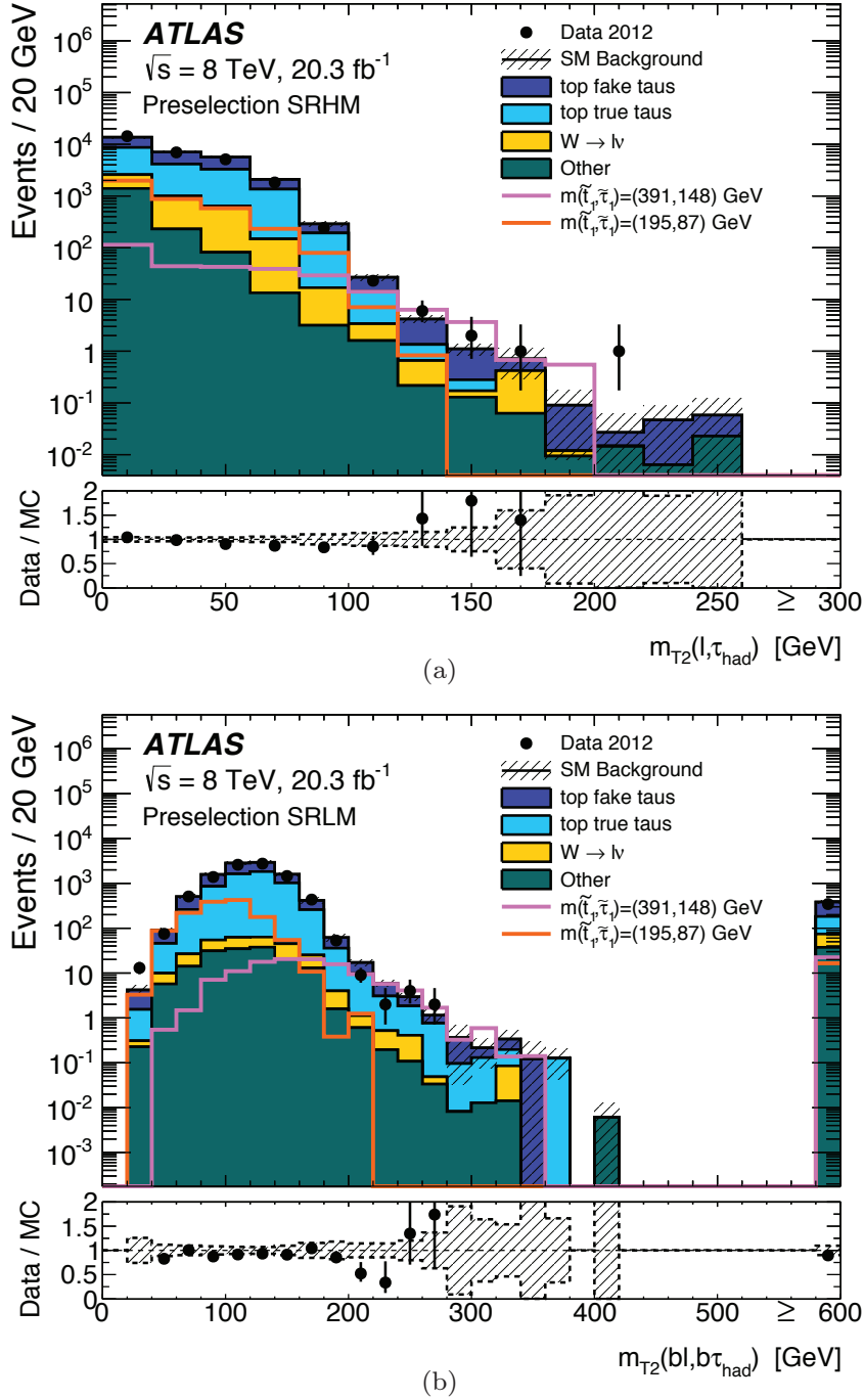
Figure 7.16: Distribution of the m_{T2}(\ell, \tau_{\text{had}}) (a) for the events passing the lep - had preselection criteria and of the m_{T2}(b\ell, b\tau_{\text{had}}) (b) for the events passing the lep - had preselection criteria with the additional requirement of a second b -tagged jet. The error band includes both statistical and systematic uncertainties. The overflow bin in the m_{T2}(b\ell, b\tau_{\text{had}}) is populated by the events that do not satisfy the m(b\ell), m(b\tau_{\text{had}}) < m_t pairing, as described in the text. Figures taken from [1].
