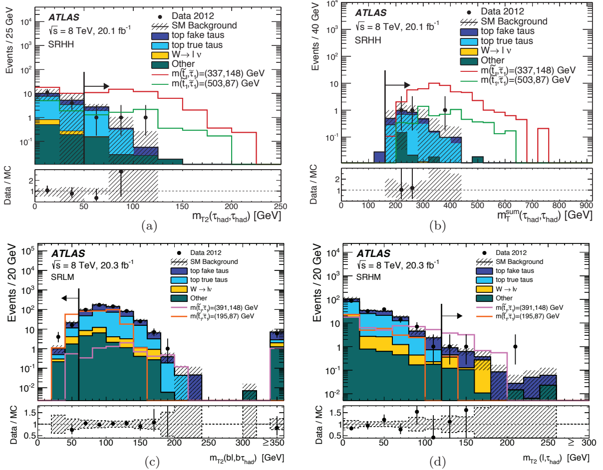
Figure 8.1: Distribution of m_{T2}(\tau_{had}, \tau_{had}) (a), m_T^{\text{sum}}(\tau_{had}, \tau_{had}) (b), m_{T2}(bl, b\tau_{had}) (c) and m_{T2}(l, \tau_{had}) (d) for all events passing the SRs criteria minus the one on the variable shown for the had-had (a,b), lep-had low-mass (c) and lep-had high-mass (d) selections, respectively. The contribution of the SM processes are stacked and the shaded area represents the total uncertainty on the prediction. The background yields have been rescaled by the post-fit normalisation scale factors. The arrows mark the cut values used to define the SR. For each distribution, two signal models are shown. Figures taken from [].
